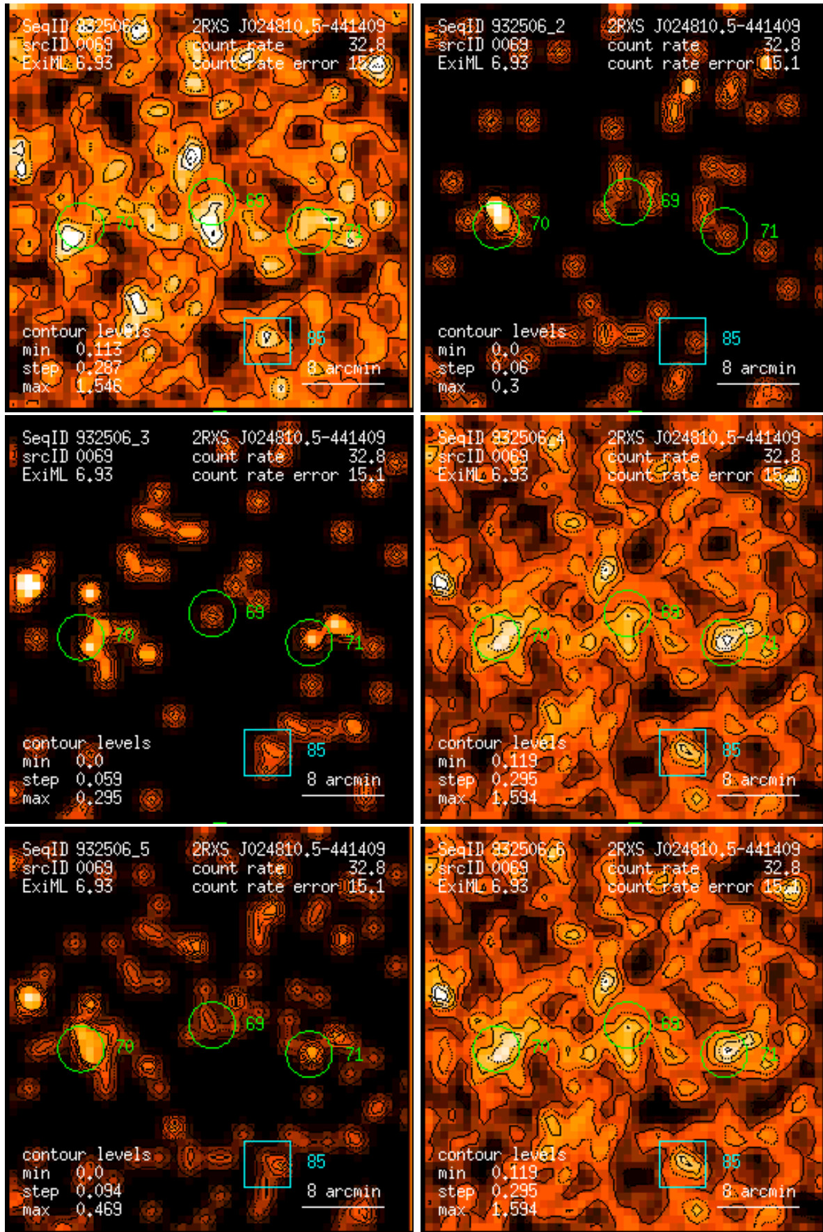
Figure 69: RASS 932506: detection 0069: band rate images, Gaussian filter: (1) PSPC channels 11 – 41, (2) 52 – 90, (3) 91 – 201, (4) 11 – 235, (5) 52 – 201, (6) 11 – 201. Broad band rates in counts/ks. Band rate contour levels in counts/ks/arcmin 2 .
