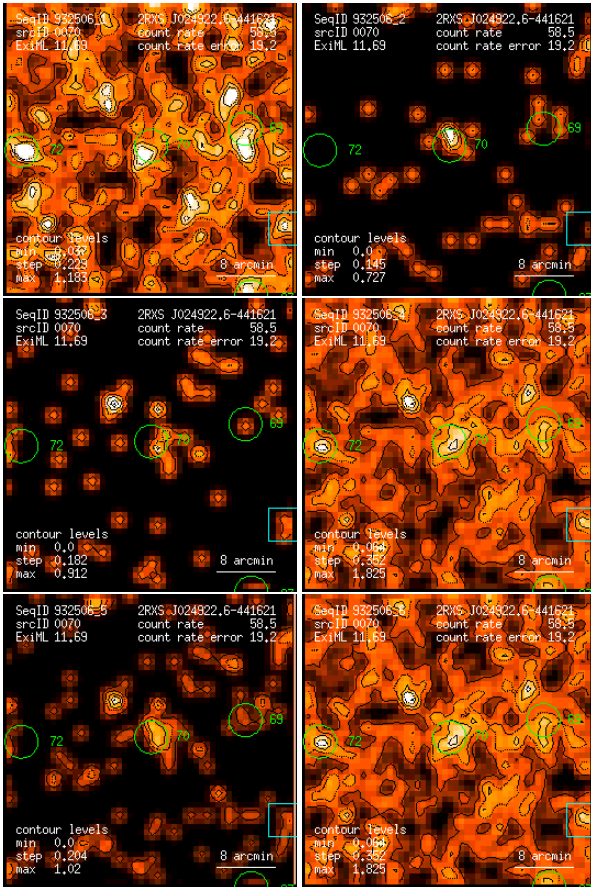
Figure 70: RASS 932506: detection 0070: band rate images, Gaussian filter: (1) PSPC channels 11 – 41, (2) 52 – 90, (3) 91 – 201, (4) 11 – 235, (5) 52 – 201, (6) 11 – 201. Broad band rates in counts/ks. Band rate contour levels in counts/ks/arcmin 2 .
