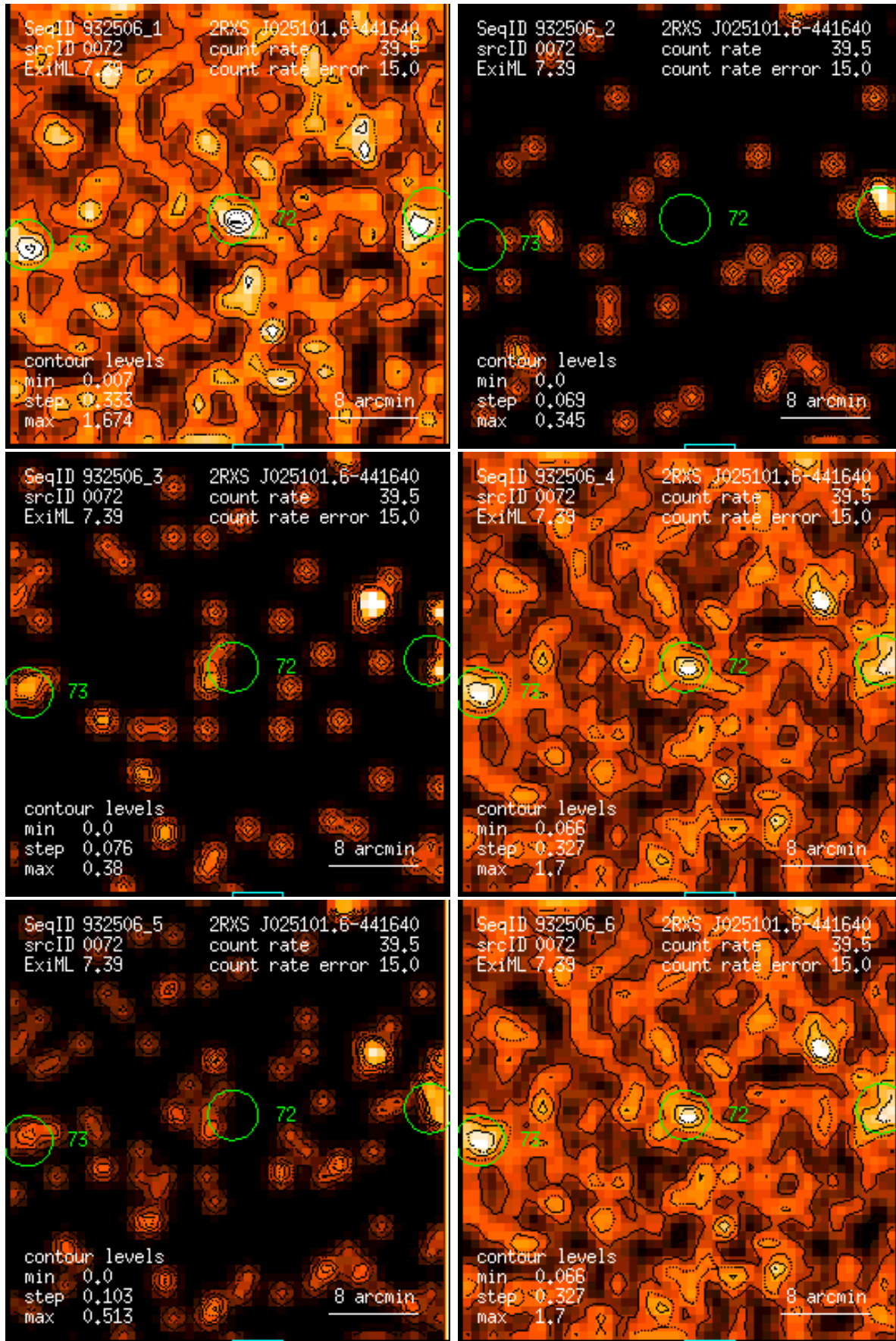
Figure 72: RASS 932506: detection 0072: band rate images, Gaussian filter: (1) PSPC channels 11 – 41, (2) 52 – 90, (3) 91 – 201, (4) 11 – 235, (5) 52 – 201, (6) 11 – 201. Broad band rates in counts/ks. Band rate contour levels in counts/ks/arcmin 2 .
