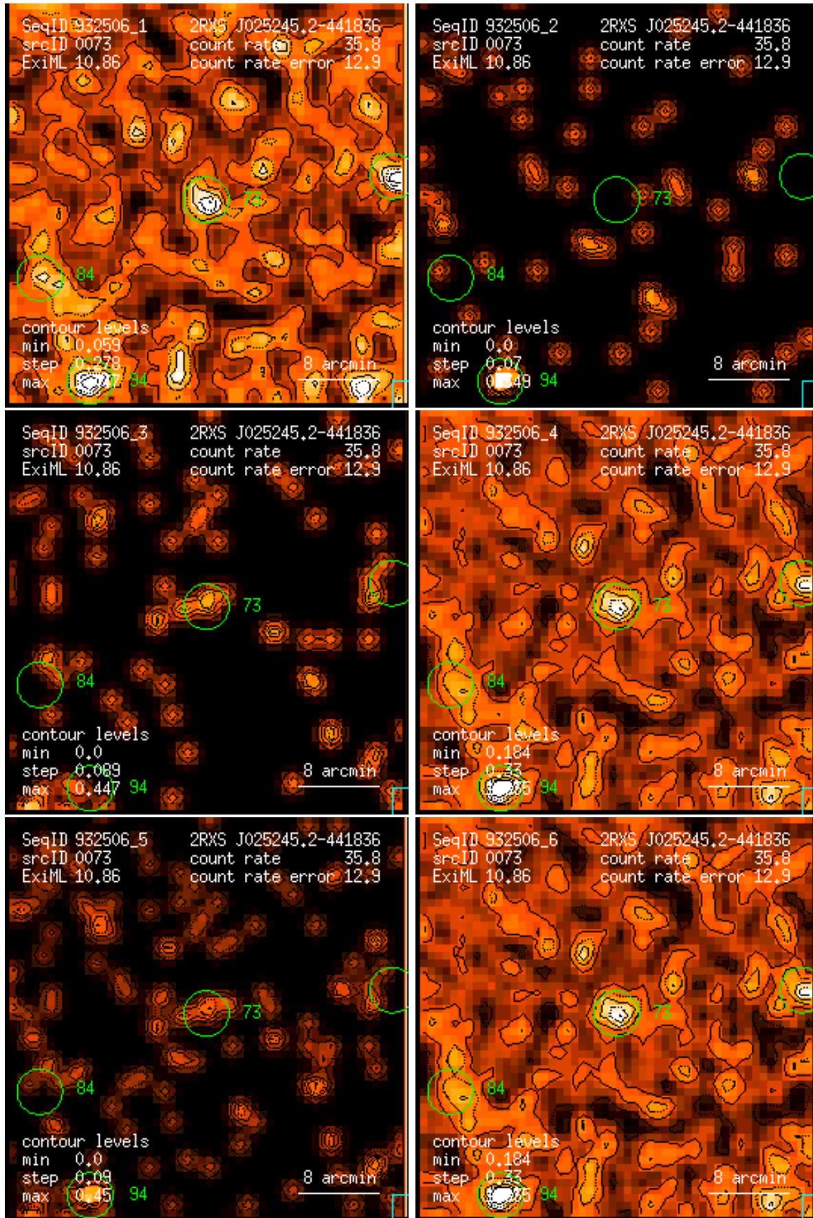
Figure 73: RASS 932506: detection 0073: band rate images, Gaussian filter: (1) PSPC channels 11 – 41, (2) 52 – 90, (3) 91 – 201, (4) 11 – 235, (5) 52 – 201, (6) 11 – 201. Broad band rates in counts/ks. Band rate contour levels in counts/ks/arcmin 2 .
