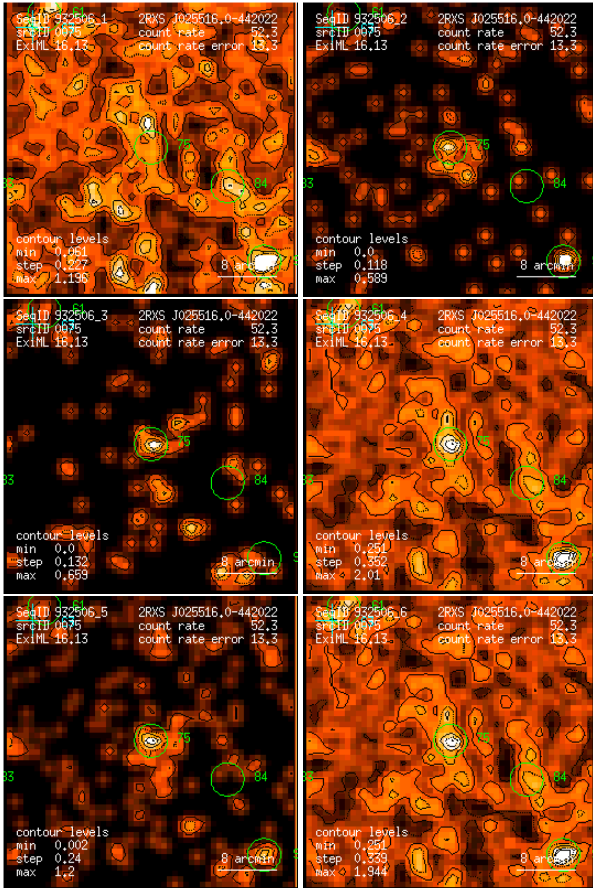
Figure 75: RASS 932506: detection 0075: band rate images, Gaussian filter: (1) PSPC channels 11 – 41, (2) 52 – 90, (3) 91 – 201, (4) 11 – 235, (5) 52 – 201, (6) 11 – 201. Broad band rates in counts/ks. Band rate contour levels in counts/ks/arcmin 2 .
