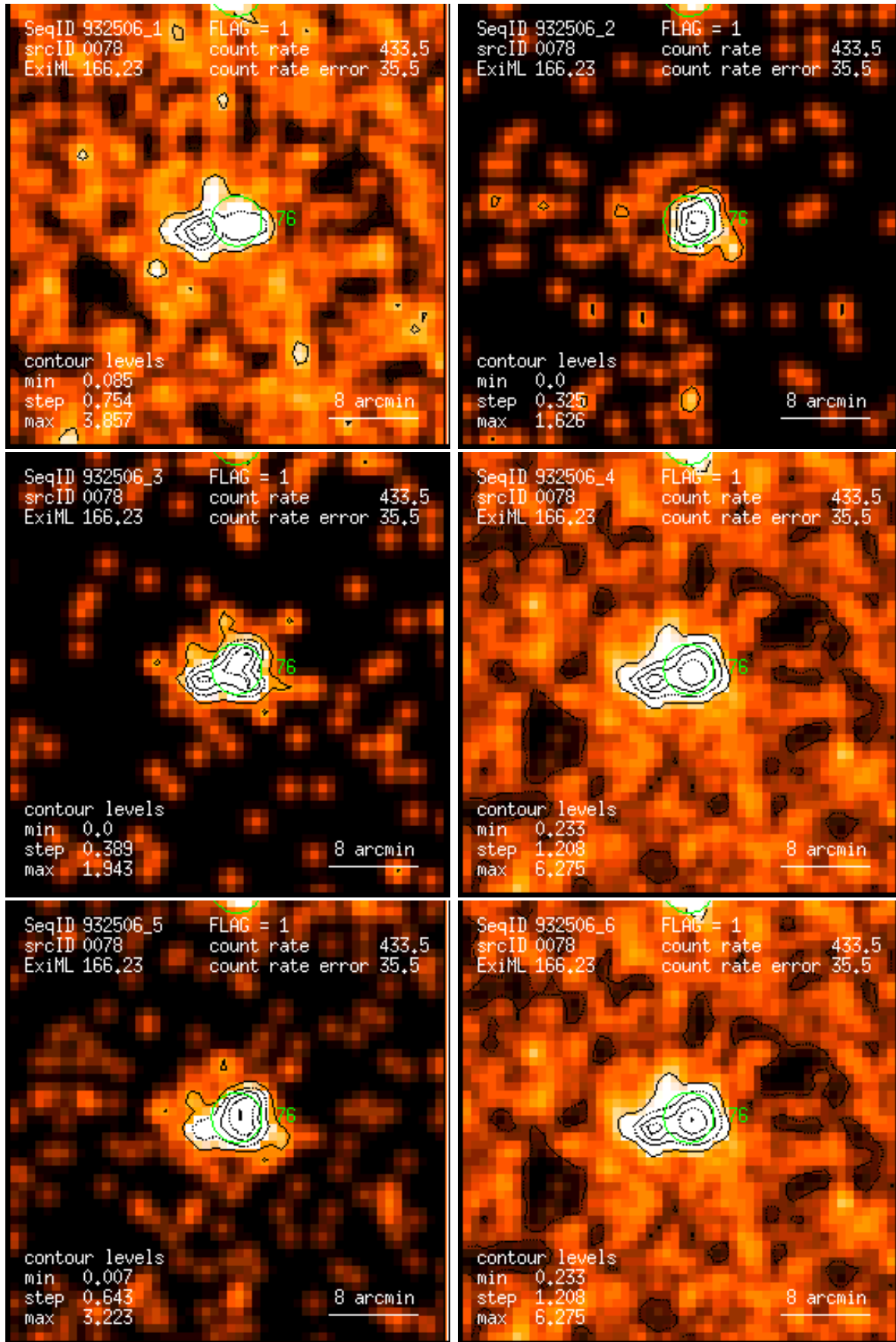
Figure 78: RASS 932506: detection 0078: band rate images, Gaussian filter: (1) PSPC channels 11 – 41, (2) 52 – 90, (3) 91 – 201, (4) 11 – 235, (5) 52 – 201, (6) 11 – 201. Broad band rates in counts/ks. Band rate contour levels in counts/ks/arcmin 2 .
