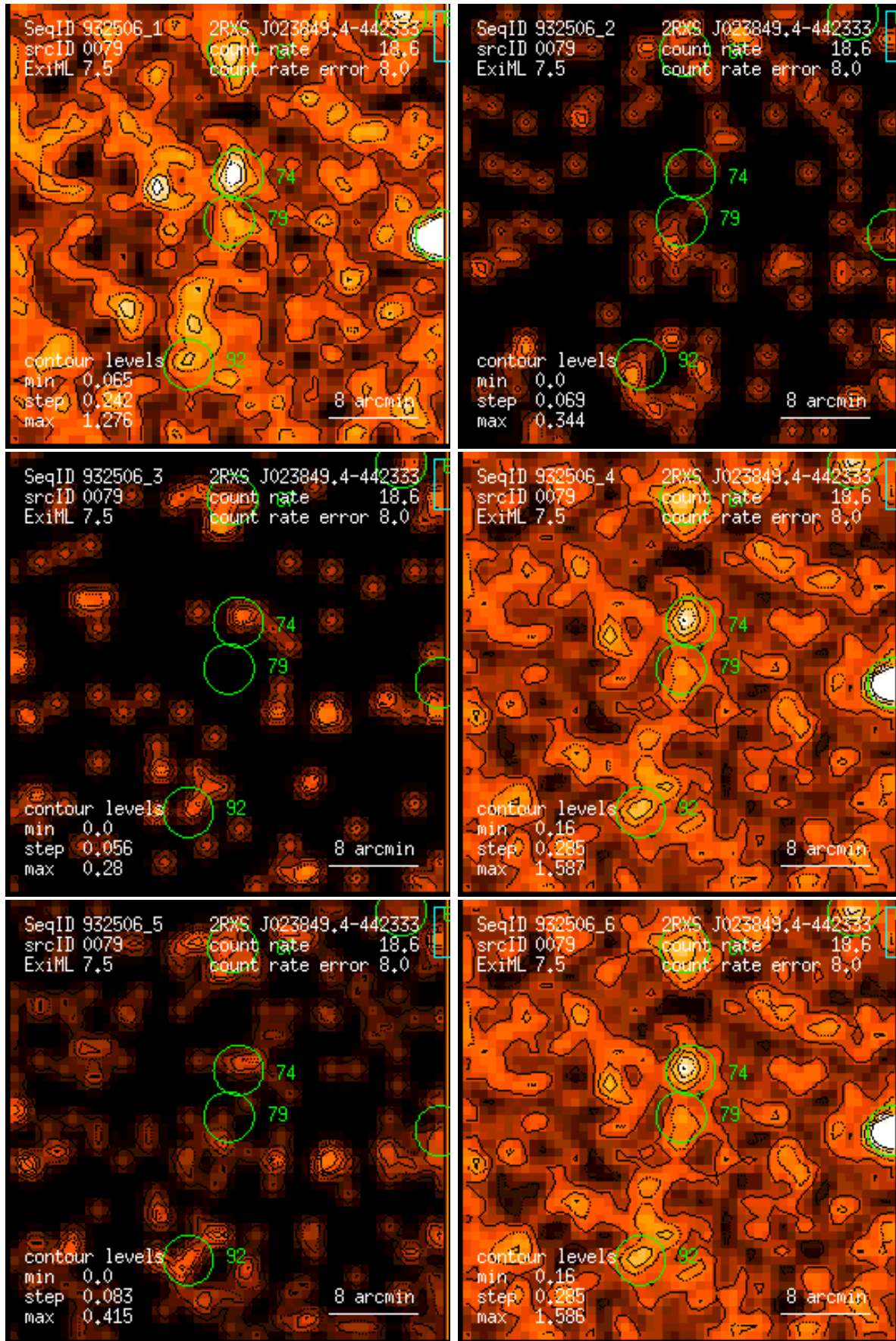
Figure 79: RASS 932506: detection 0079: band rate images, Gaussian filter: (1) PSPC channels 11 – 41, (2) 52 – 90, (3) 91 – 201, (4) 11 – 235, (5) 52 – 201, (6) 11 – 201. Broad band rates in counts/ks. Band rate contour levels in counts/ks/arcmin 2 .
