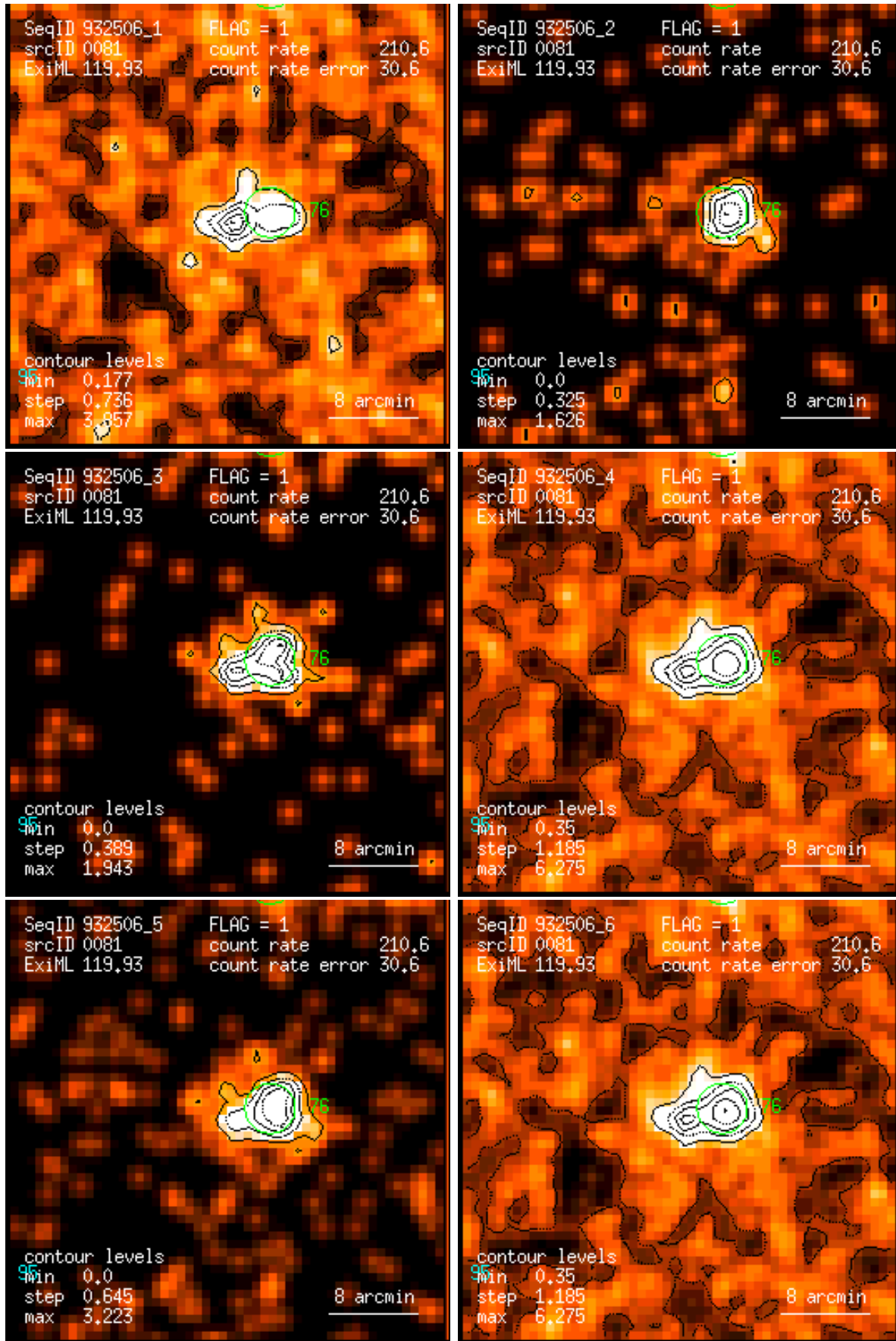
Figure 81: RASS 932506: detection 0081: band rate images, Gaussian filter: (1) PSPC channels 11 – 41, (2) 52 – 90, (3) 91 – 201, (4) 11 – 235, (5) 52 – 201, (6) 11 – 201. Broad band rates in counts/ks. Band rate contour levels in counts/ks/arcmin 2 .
