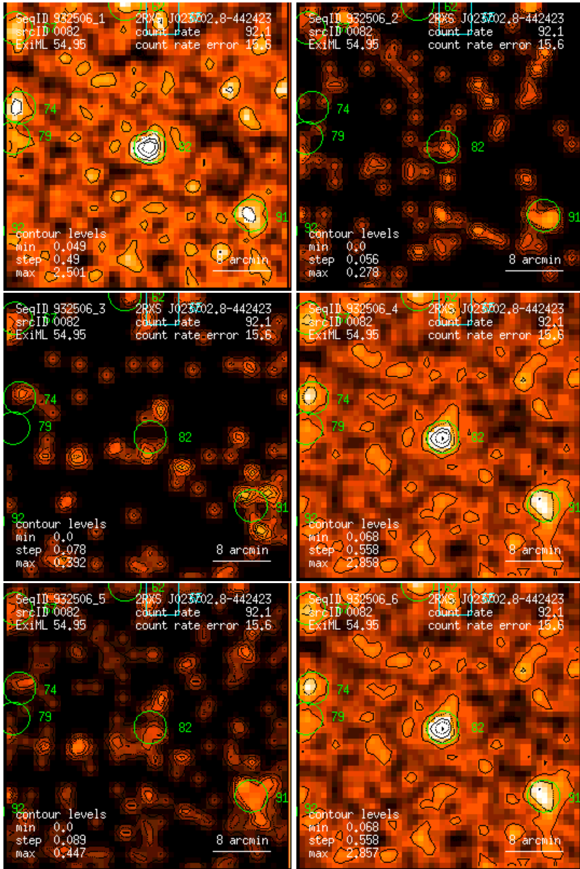
Figure 82: RASS 932506: detection 0082: band rate images, Gaussian filter: (1) PSPC channels 11 – 41, (2) 52 – 90, (3) 91 – 201, (4) 11 – 235, (5) 52 – 201, (6) 11 – 201. Broad band rates in counts/ks. Band rate contour levels in counts/ks/arcmin 2 .
