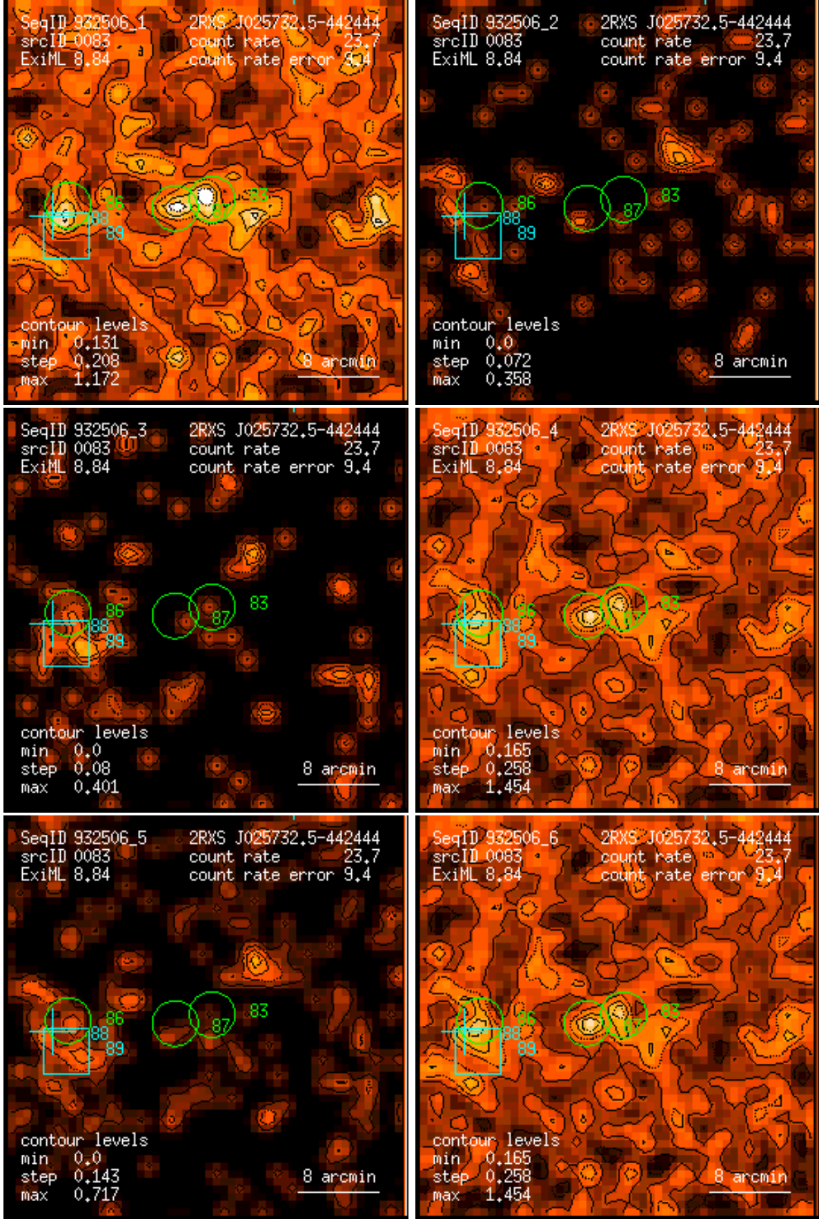
Figure 83: RASS 932506: detection 0083: band rate images, Gaussian filter: (1) PSPC channels 11 – 41, (2) 52 – 90, (3) 91 – 201, (4) 11 – 235, (5) 52 – 201, (6) 11 – 201. Broad band rates in counts/ks. Band rate contour levels in counts/ks/arcmin 2 .
