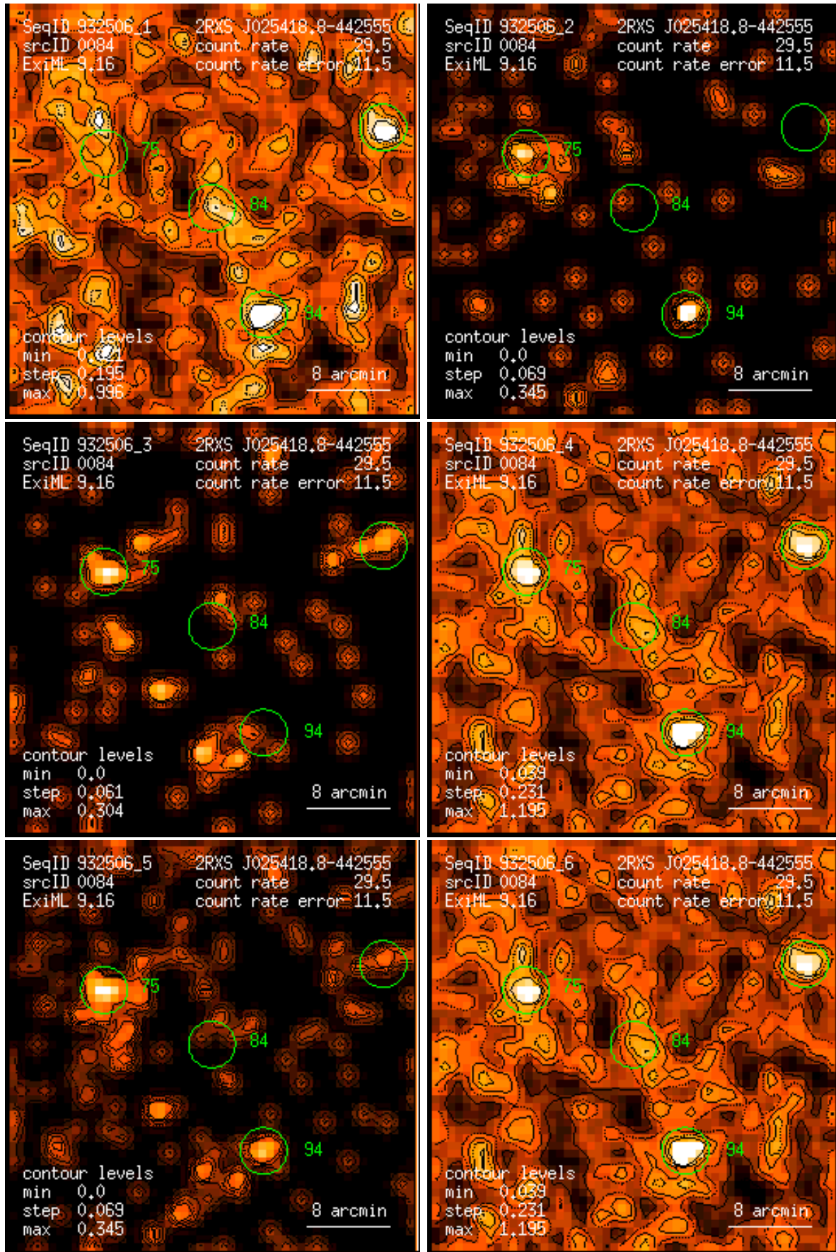
Figure 84: RASS 932506: detection 0084: band rate images, Gaussian filter: (1) PSPC channels 11 – 41, (2) 52 – 90, (3) 91 – 201, (4) 11 – 235, (5) 52 – 201, (6) 11 – 201. Broad band rates in counts/ks. Band rate contour levels in counts/ks/arcmin 2 .
