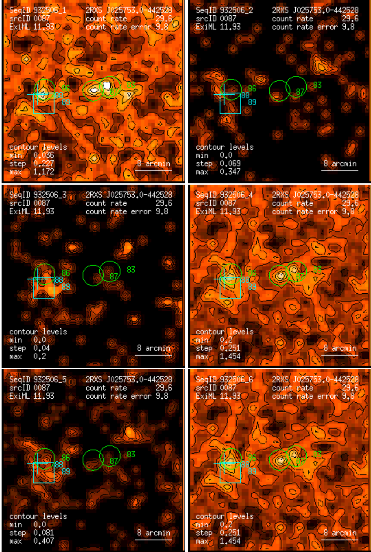
Figure 87: RASS 932506: detection 0087: band rate images, Gaussian filter: (1) PSPC channels 11 – 41, (2) 52 – 90, (3) 91 – 201, (4) 11 – 235, (5) 52 – 201, (6) 11 – 201. Broad band rates in counts/ks. Band rate contour levels in counts/ks/arcmin 2 .
