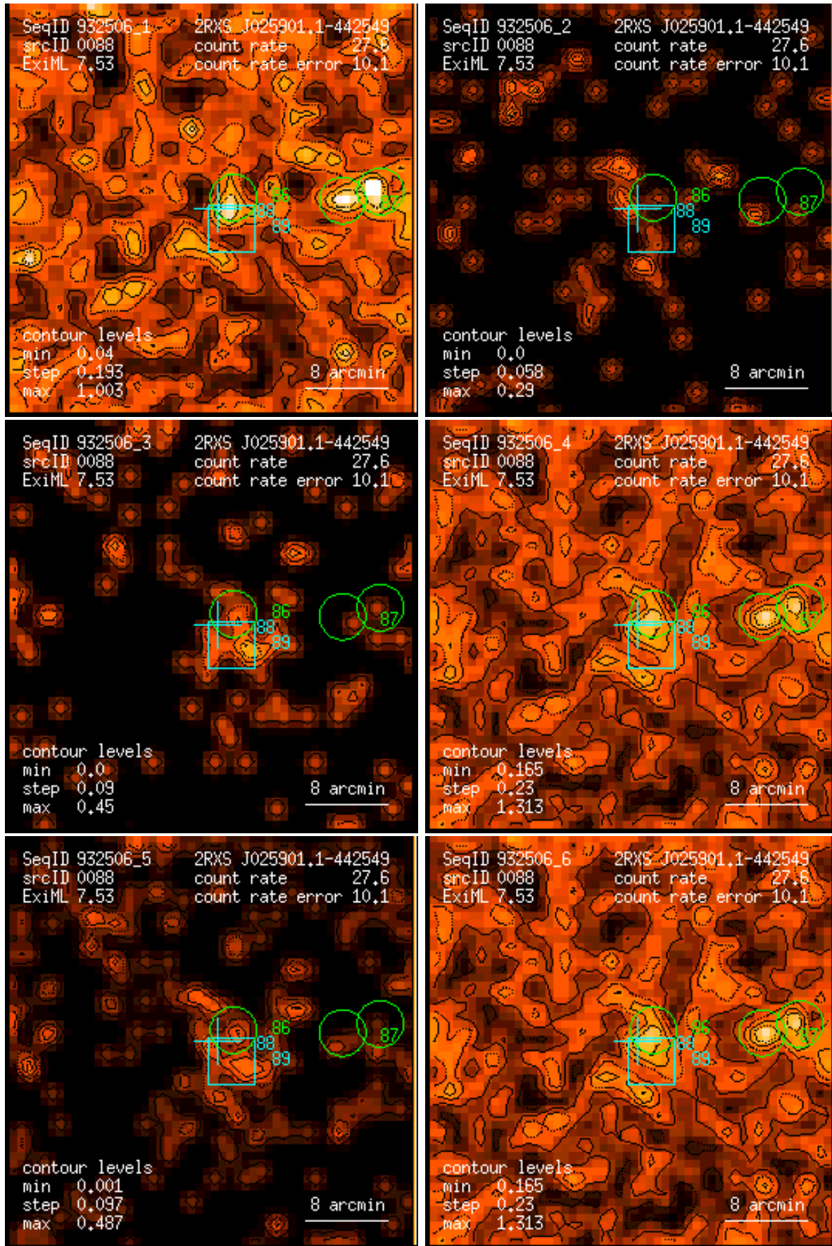
Figure 88: RASS 932506: detection 0088: band rate images, Gaussian filter: (1) PSPC channels 11 – 41, (2) 52 – 90, (3) 91 – 201, (4) 11 – 235, (5) 52 – 201, (6) 11 – 201. Broad band rates in counts/ks. Band rate contour levels in counts/ks/arcmin 2 .
