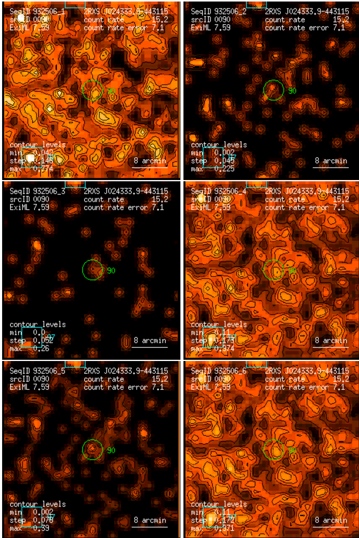
Figure 90: RASS 932506: detection 0090: band rate images, Gaussian filter: (1) PSPC channels 11 – 41, (2) 52 – 90, (3) 91 – 201, (4) 11 – 235, (5) 52 – 201, (6) 11 – 201. Broad band rates in counts/ks. Band rate contour levels in counts/ks/arcmin 2 .
