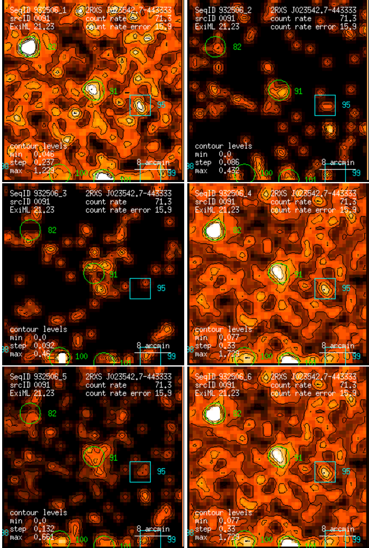
Figure 91: RASS 932506: detection 0091: band rate images, Gaussian filter: (1) PSPC channels 11 – 41, (2) 52 – 90, (3) 91 – 201, (4) 11 – 235, (5) 52 – 201, (6) 11 – 201. Broad band rates in counts/ks. Band rate contour levels in counts/ks/arcmin 2 .
