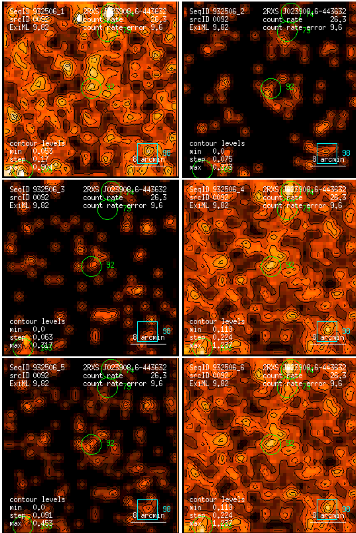
Figure 92: RASS 932506: detection 0092: band rate images, Gaussian filter: (1) PSPC channels 11 – 41, (2) 52 – 90, (3) 91 – 201, (4) 11 – 235, (5) 52 – 201, (6) 11 – 201. Broad band rates in counts/ks. Band rate contour levels in counts/ks/arcmin 2 .
