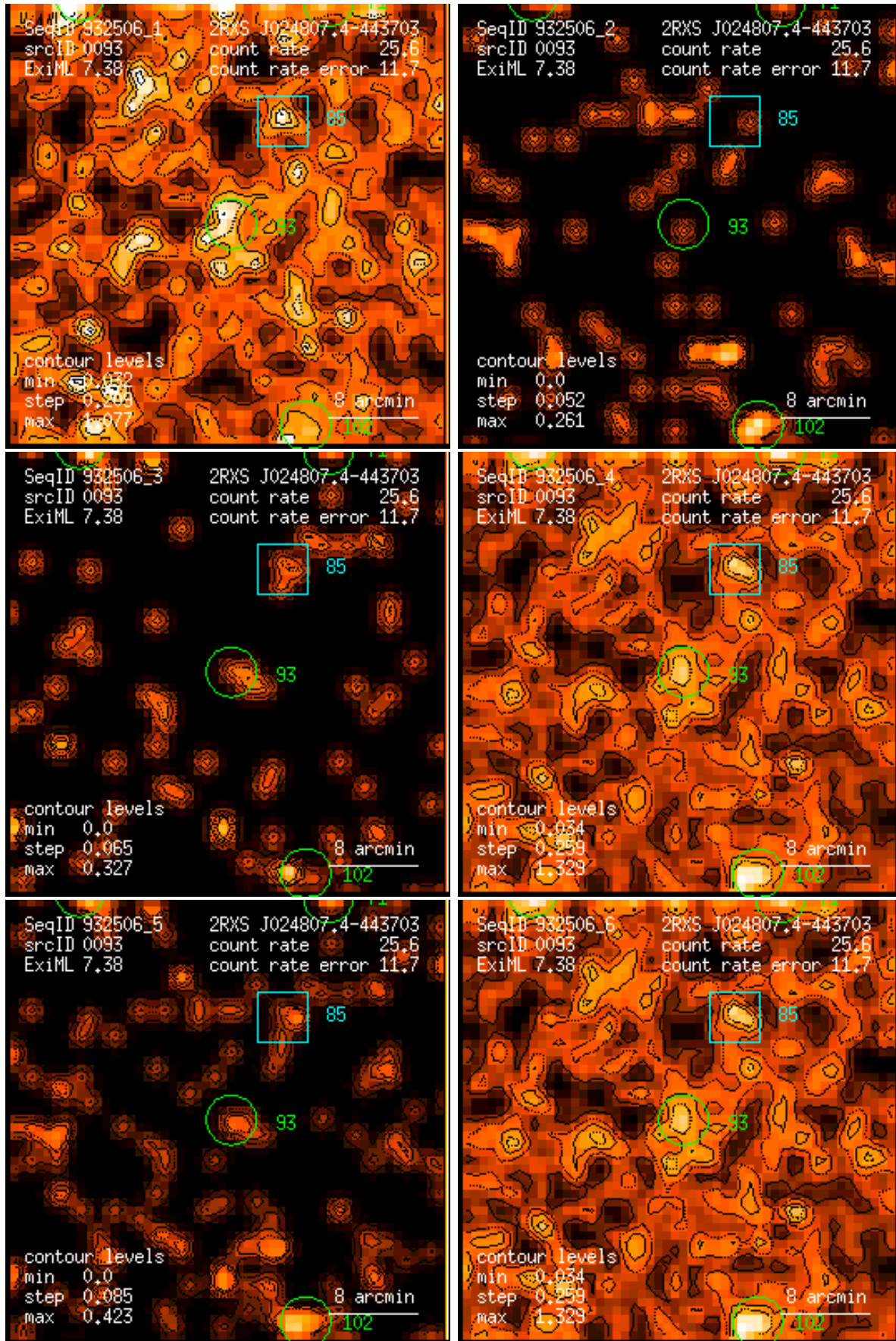
Figure 93: RASS 932506: detection 0093: band rate images, Gaussian filter: (1) PSPC channels 11 – 41, (2) 52 – 90, (3) 91 – 201, (4) 11 – 235, (5) 52 – 201, (6) 11 – 201. Broad band rates in counts/ks. Band rate contour levels in counts/ks/arcmin 2 .
