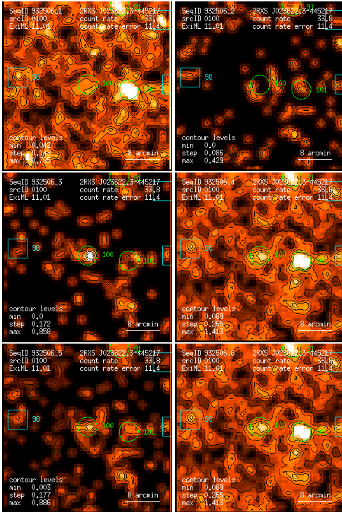
Figure 100: RASS 932506: detection 0100: band rate images, Gaussian filter: (1) PSPC channels 11 – 41, (2) 52 – 90, (3) 91 – 201, (4) 11 – 235, (5) 52 – 201, (6) 11 – 201. Broad band rates in counts/ks. Band rate contour levels in counts/ks/arcmin 2 .
