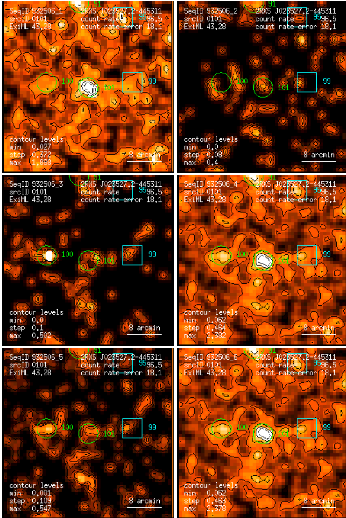
Figure 101: RASS 932506: detection 0101: band rate images, Gaussian filter: (1) PSPC channels 11 – 41, (2) 52 – 90, (3) 91 – 201, (4) 11 – 235, (5) 52 – 201, (6) 11 – 201. Broad band rates in counts/ks. Band rate contour levels in counts/ks/arcmin 2 .
