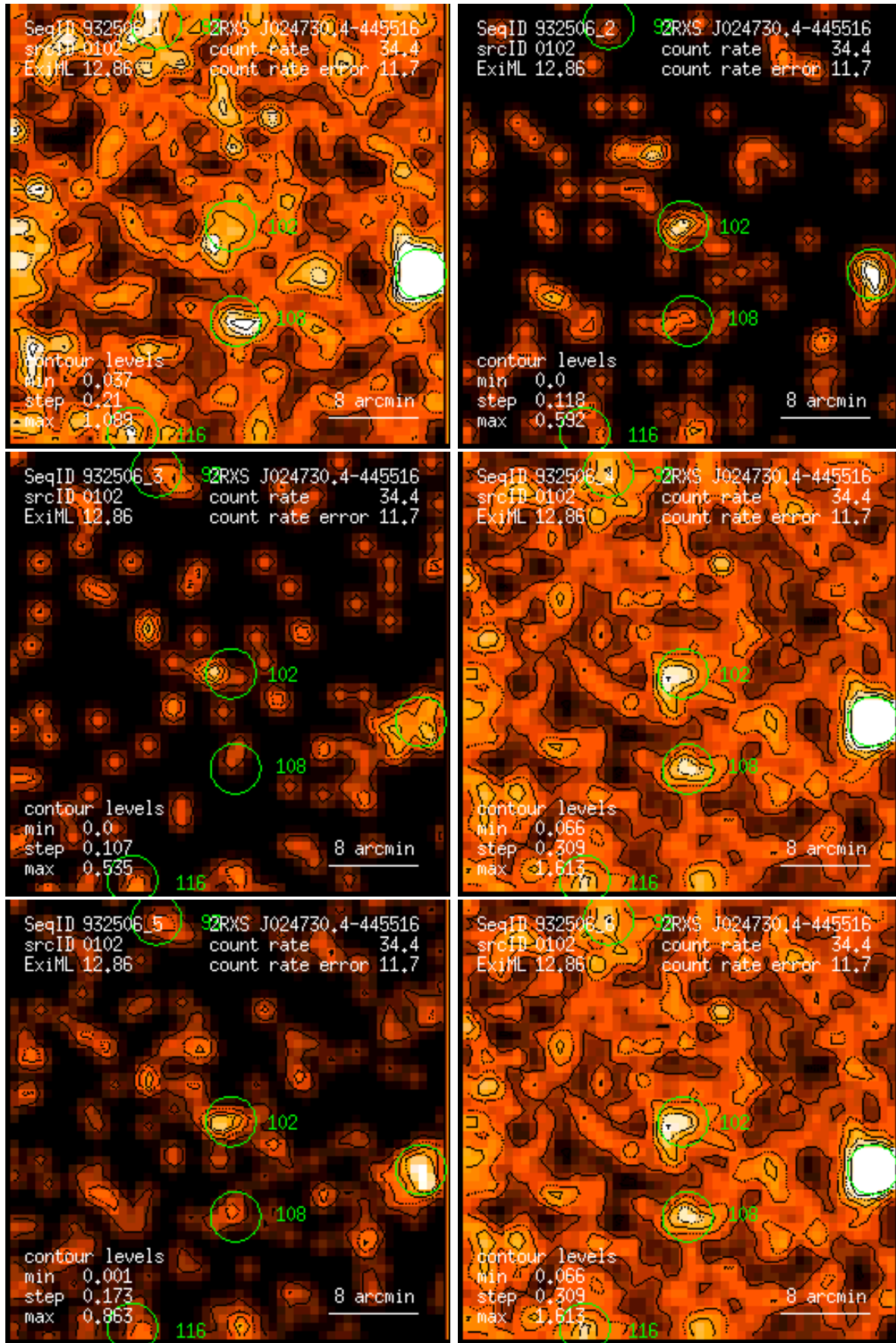
Figure 102: RASS 932506: detection 0102: band rate images, Gaussian filter: (1) PSPC channels 11 – 41, (2) 52 – 90, (3) 91 – 201, (4) 11 – 235, (5) 52 – 201, (6) 11 – 201. Broad band rates in counts/ks. Band rate contour levels in counts/ks/arcmin 2 .
