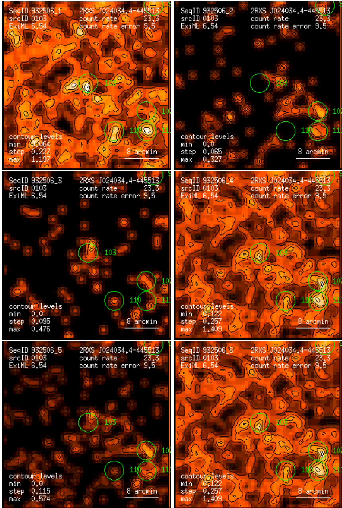
Figure 103: RASS 932506: detection 0103: band rate images, Gaussian filter: (1) PSPC channels 11 – 41, (2) 52 – 90, (3) 91 – 201, (4) 11 – 235, (5) 52 – 201, (6) 11 – 201. Broad band rates in counts/ks. Band rate contour levels in counts/ks/arcmin 2 .
