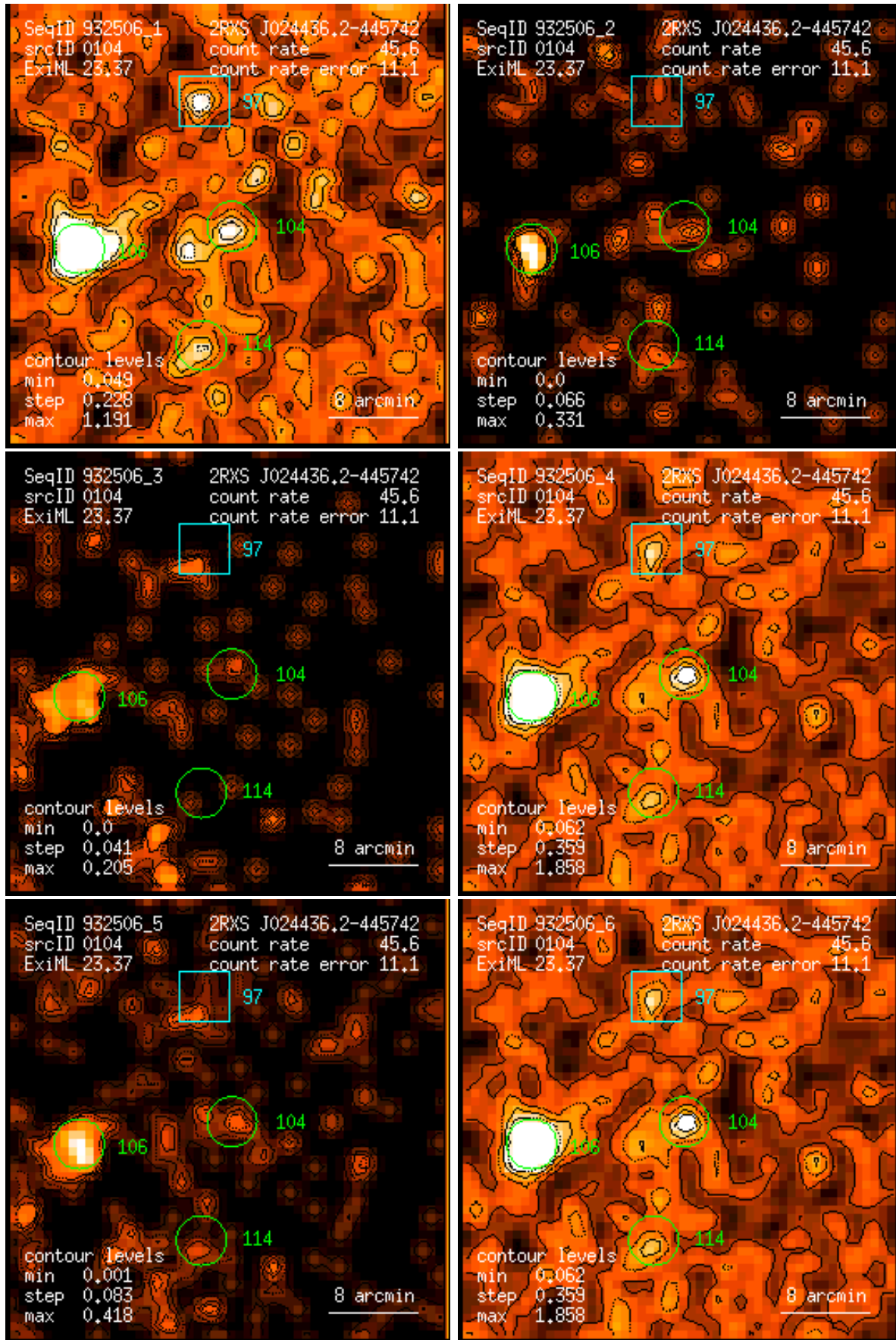
Figure 104: RASS 932506: detection 0104: band rate images, Gaussian filter: (1) PSPC channels 11 – 41, (2) 52 – 90, (3) 91 – 201, (4) 11 – 235, (5) 52 – 201, (6) 11 – 201. Broad band rates in counts/ks. Band rate contour levels in counts/ks/arcmin 2 .
