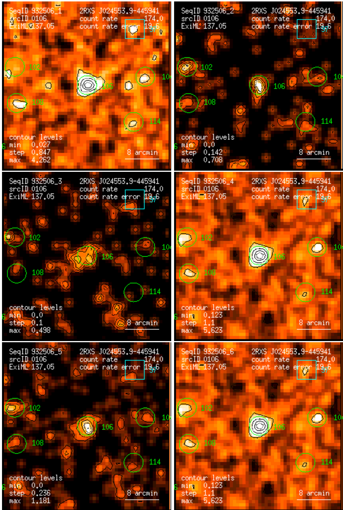
Figure 106: RASS 932506: detection 0106: band rate images, Gaussian filter: (1) PSPC channels 11 – 41, (2) 52 – 90, (3) 91 – 201, (4) 11 – 235, (5) 52 – 201, (6) 11 – 201. Broad band rates in counts/ks. Band rate contour levels in counts/ks/arcmin 2 .
