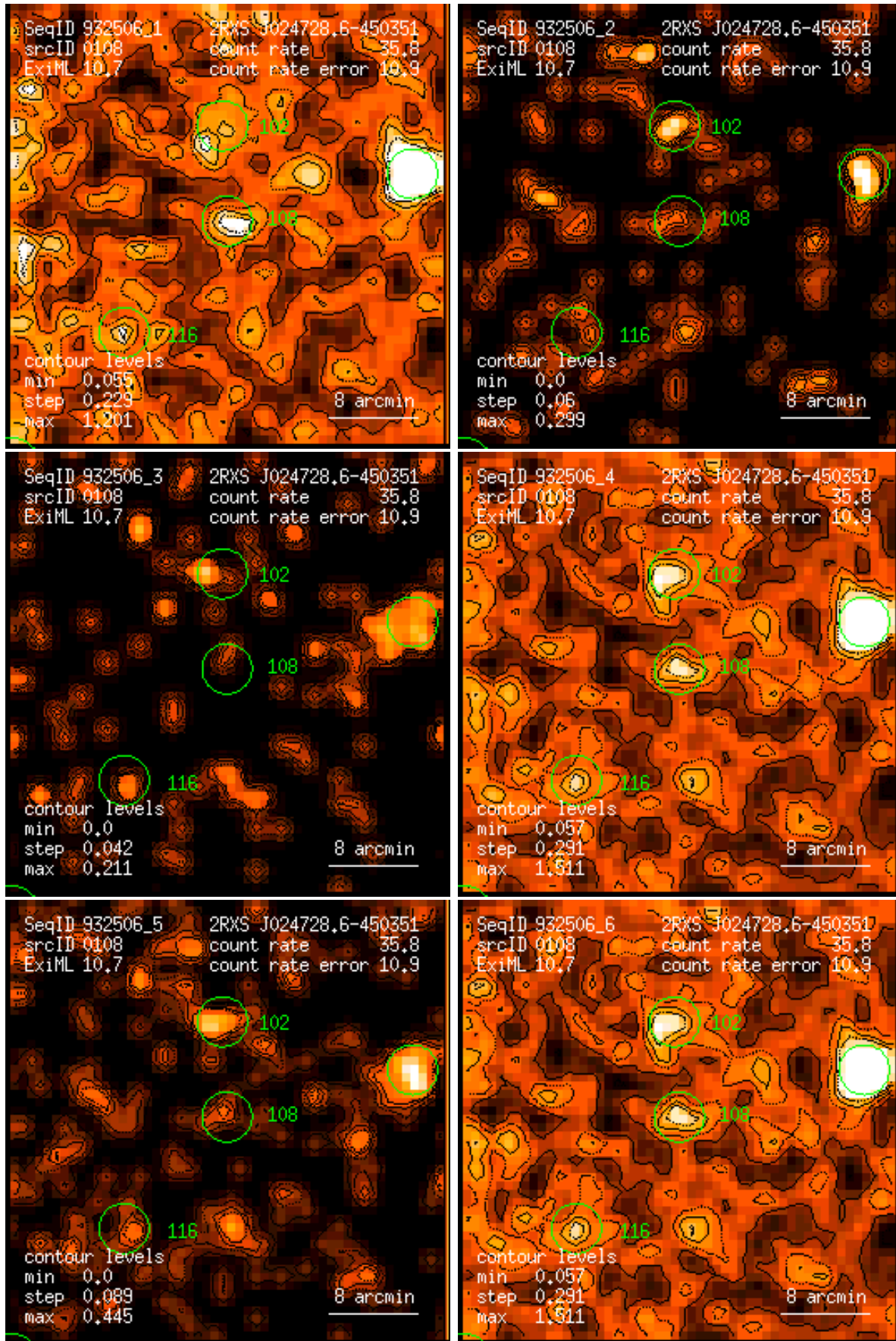
Figure 108: RASS 932506: detection 0108: band rate images, Gaussian filter: (1) PSPC channels 11 – 41, (2) 52 – 90, (3) 91 – 201, (4) 11 – 235, (5) 52 – 201, (6) 11 – 201. Broad band rates in counts/ks. Band rate contour levels in counts/ks/arcmin 2 .
