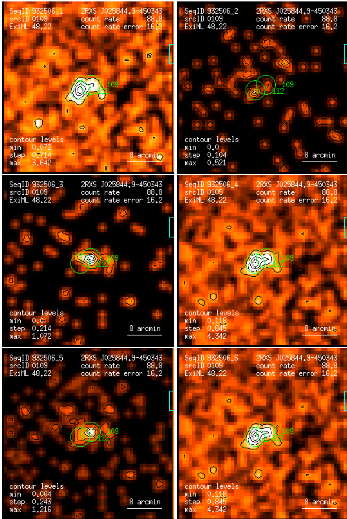
Figure 109: RASS 932506: detection 0109: band rate images, Gaussian filter: (1) PSPC channels 11 – 41, (2) 52 – 90, (3) 91 – 201, (4) 11 – 235, (5) 52 – 201, (6) 11 – 201. Broad band rates in counts/ks. Band rate contour levels in counts/ks/arcmin 2 .
