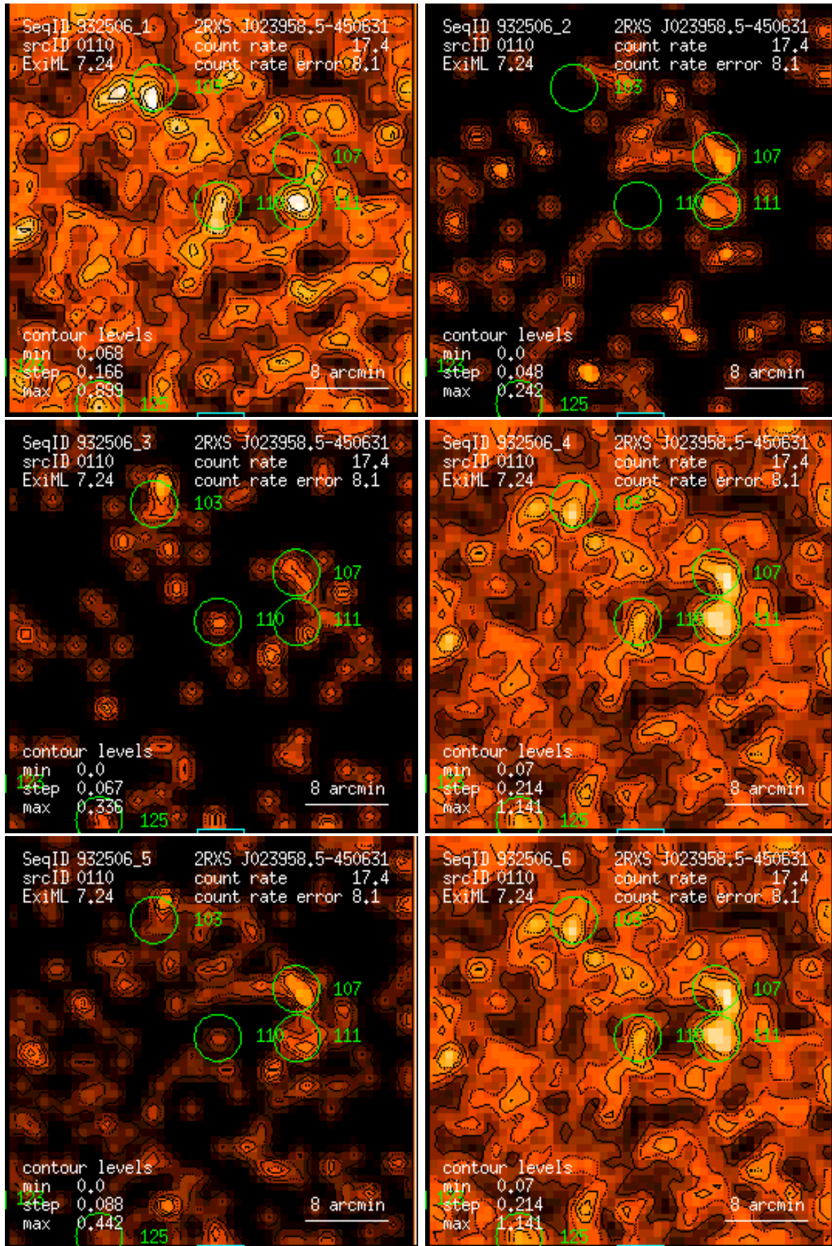
Figure 110: RASS 932506: detection 0110: band rate images, Gaussian filter: (1) PSPC channels 11 – 41, (2) 52 – 90, (3) 91 – 201, (4) 11 – 235, (5) 52 – 201, (6) 11 – 201. Broad band rates in counts/ks. Band rate contour levels in counts/ks/arcmin 2 .
