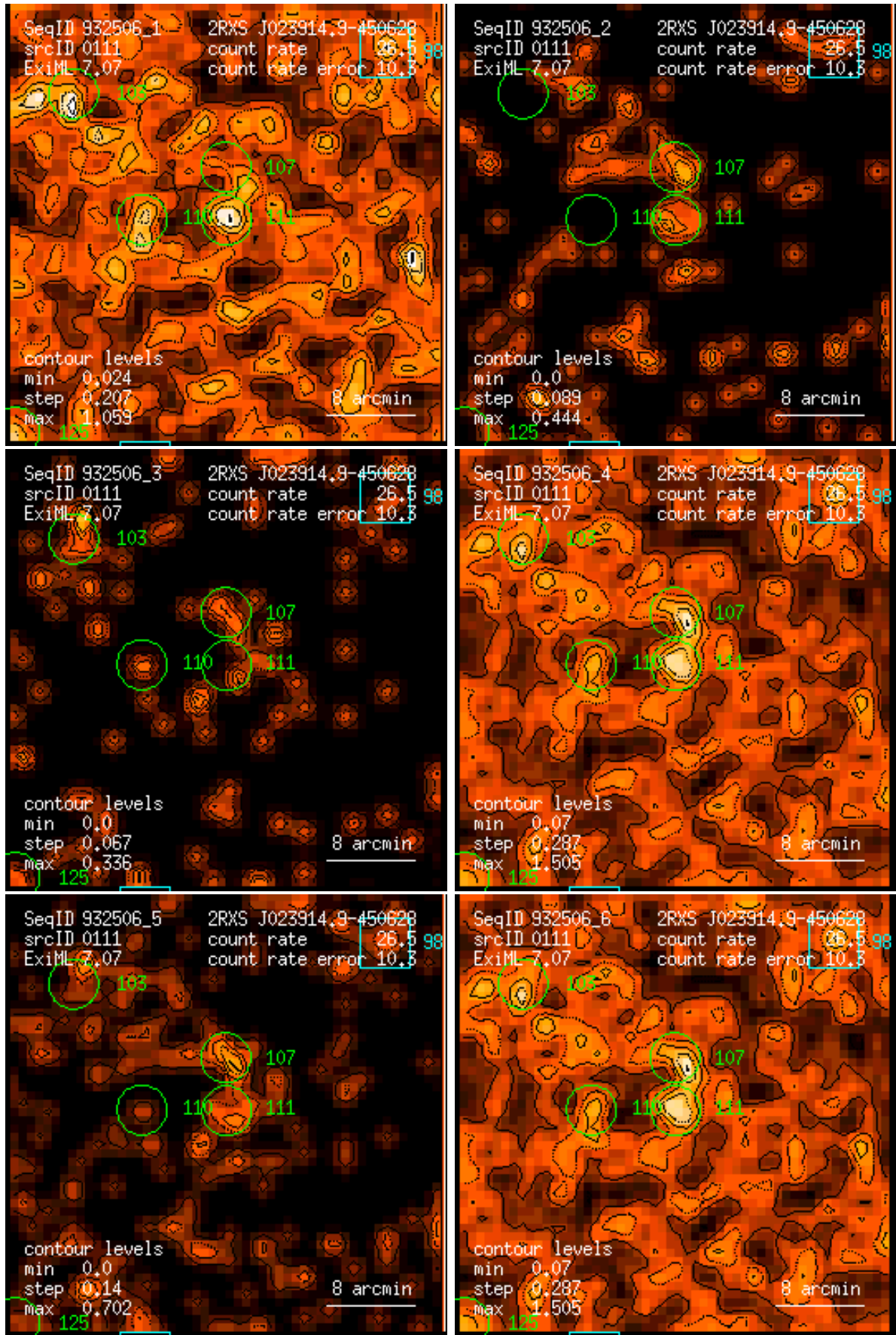
Figure 111: RASS 932506: detection 0111: band rate images, Gaussian filter: (1) PSPC channels 11 – 41, (2) 52 – 90, (3) 91 – 201, (4) 11 – 235, (5) 52 – 201, (6) 11 – 201. Broad band rates in counts/ks. Band rate contour levels in counts/ks/arcmin 2 .
