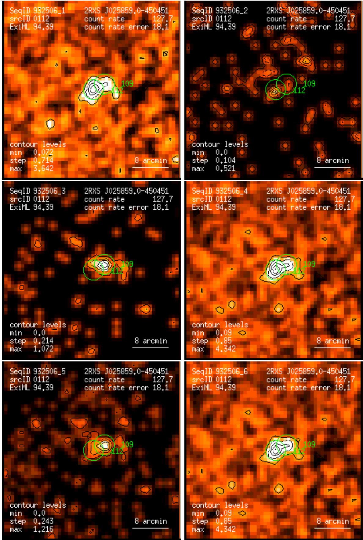
Figure 112: RASS 932506: detection 0112: band rate images, Gaussian filter: (1) PSPC channels 11 – 41, (2) 52 – 90, (3) 91 – 201, (4) 11 – 235, (5) 52 – 201, (6) 11 – 201. Broad band rates in counts/ks. Band rate contour levels in counts/ks/arcmin 2 .
