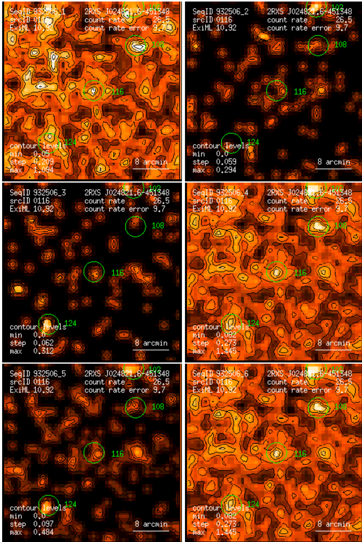
Figure 116: RASS 932506: detection 0116: band rate images, Gaussian filter: (1) PSPC channels 11 – 41, (2) 52 – 90, (3) 91 – 201, (4) 11 – 235, (5) 52 – 201, (6) 11 – 201. Broad band rates in counts/ks. Band rate contour levels in counts/ks/arcmin 2 .
