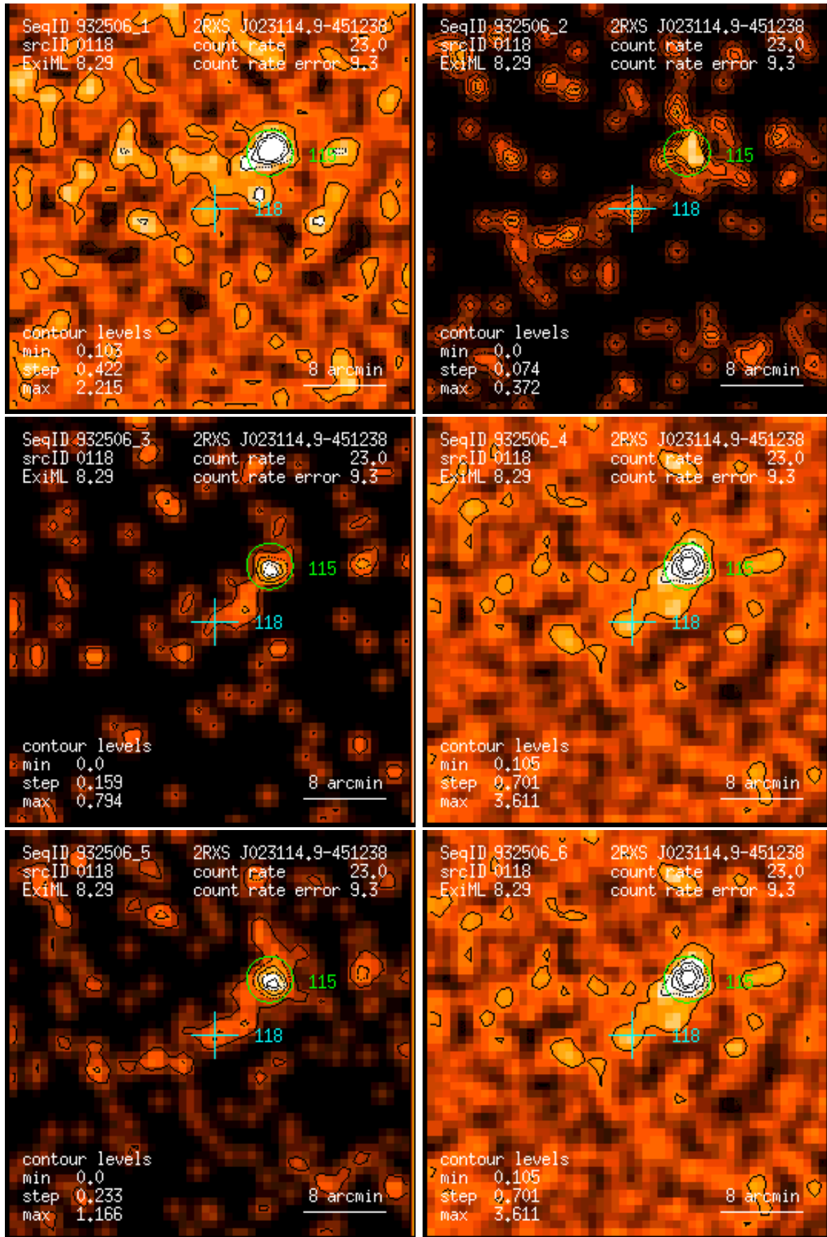
Figure 118: RASS 932506: detection 0118: band rate images, Gaussian filter: (1) PSPC channels 11 – 41, (2) 52 – 90, (3) 91 – 201, (4) 11 – 235, (5) 52 – 201, (6) 11 – 201. Broad band rates in counts/ks. Band rate contour levels in counts/ks/arcmin 2 .
