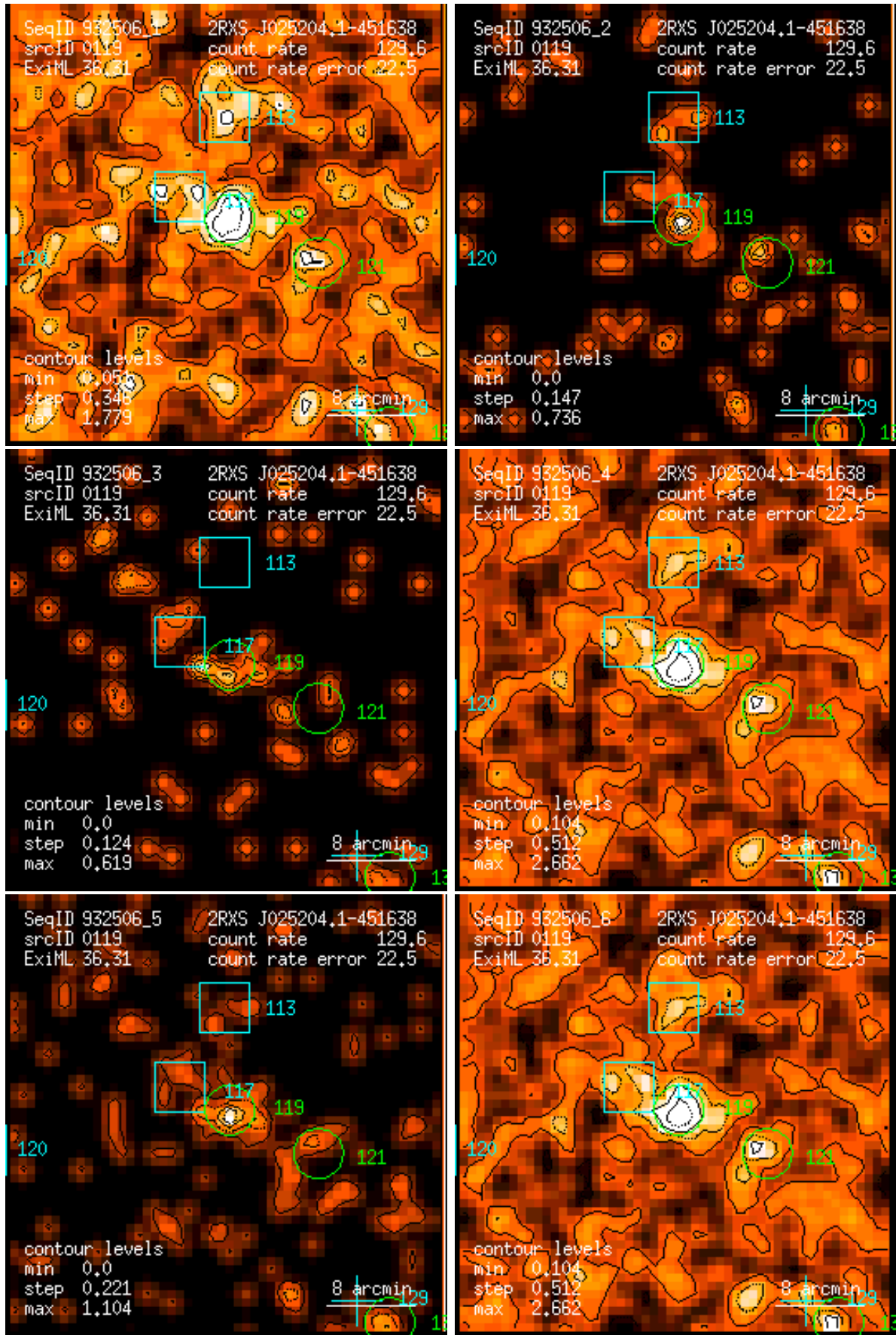
Figure 119: RASS 932506: detection 0119: band rate images, Gaussian filter: (1) PSPC channels 11 – 41, (2) 52 – 90, (3) 91 – 201, (4) 11 – 235, (5) 52 – 201, (6) 11 – 201. Broad band rates in counts/ks. Band rate contour levels in counts/ks/arcmin 2 .
