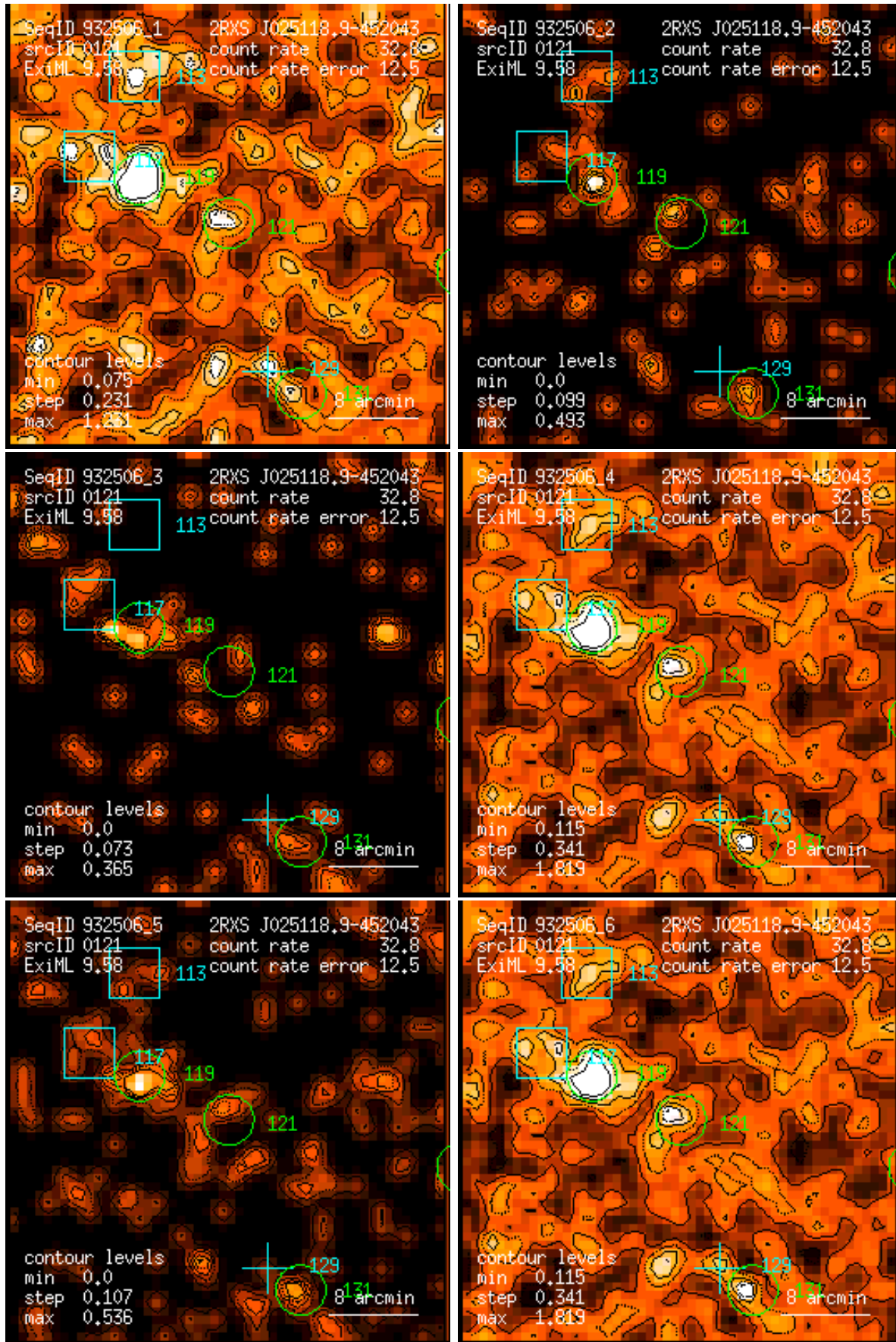
Figure 121: RASS 932506: detection 0121: band rate images, Gaussian filter: (1) PSPC channels 11 – 41, (2) 52 – 90, (3) 91 – 201, (4) 11 – 235, (5) 52 – 201, (6) 11 – 201. Broad band rates in counts/ks. Band rate contour levels in counts/ks/arcmin 2 .
