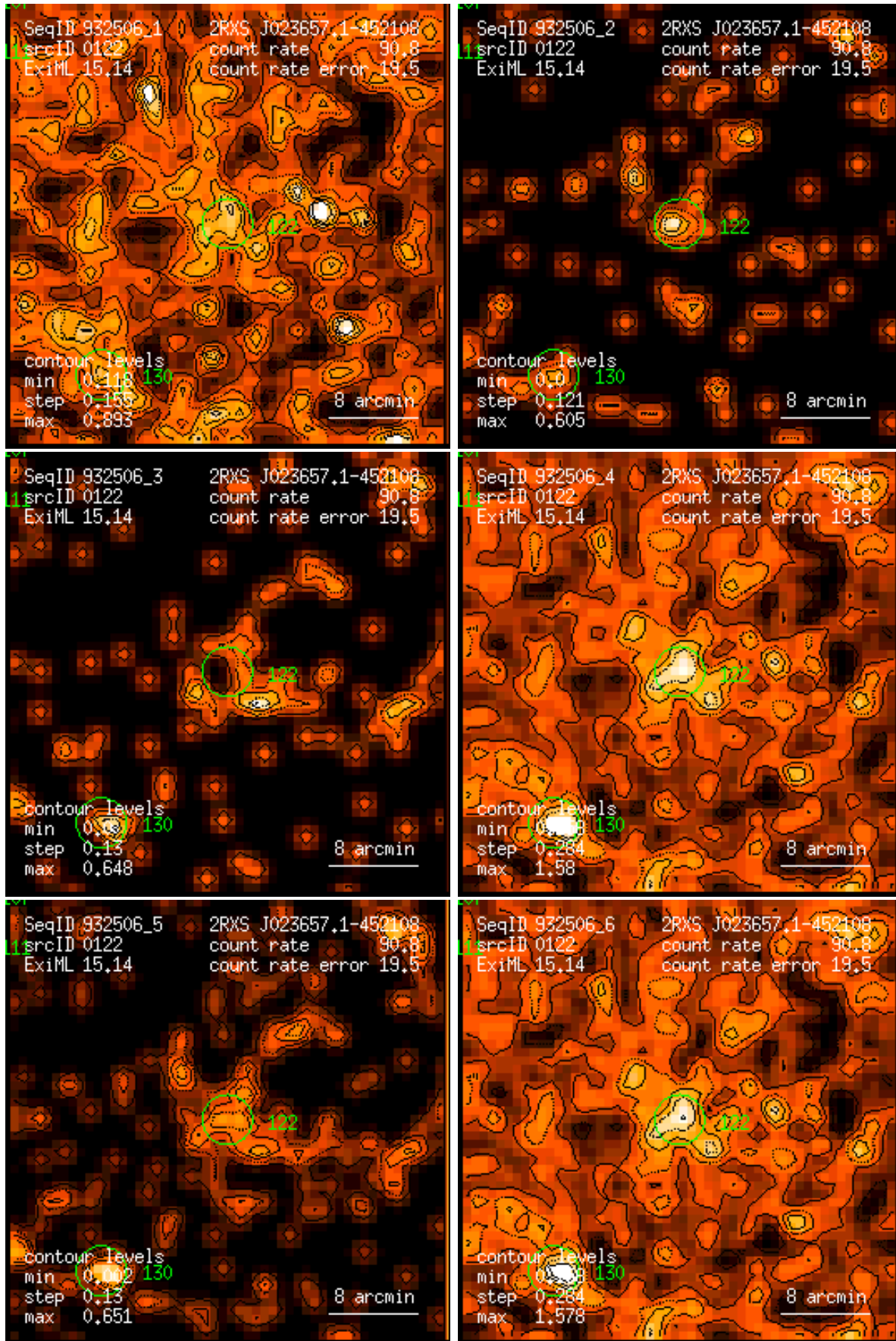
Figure 122: RASS 932506: detection 0122: band rate images, Gaussian filter: (1) PSPC channels 11 – 41, (2) 52 – 90, (3) 91 – 201, (4) 11 – 235, (5) 52 – 201, (6) 11 – 201. Broad band rates in counts/ks. Band rate contour levels in counts/ks/arcmin 2 .
