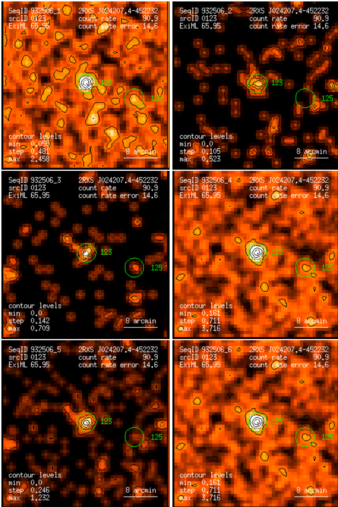
Figure 123: RASS 932506: detection 0123: band rate images, Gaussian filter: (1) PSPC channels 11 – 41, (2) 52 – 90, (3) 91 – 201, (4) 11 – 235, (5) 52 – 201, (6) 11 – 201. Broad band rates in counts/ks. Band rate contour levels in counts/ks/arcmin 2 .
