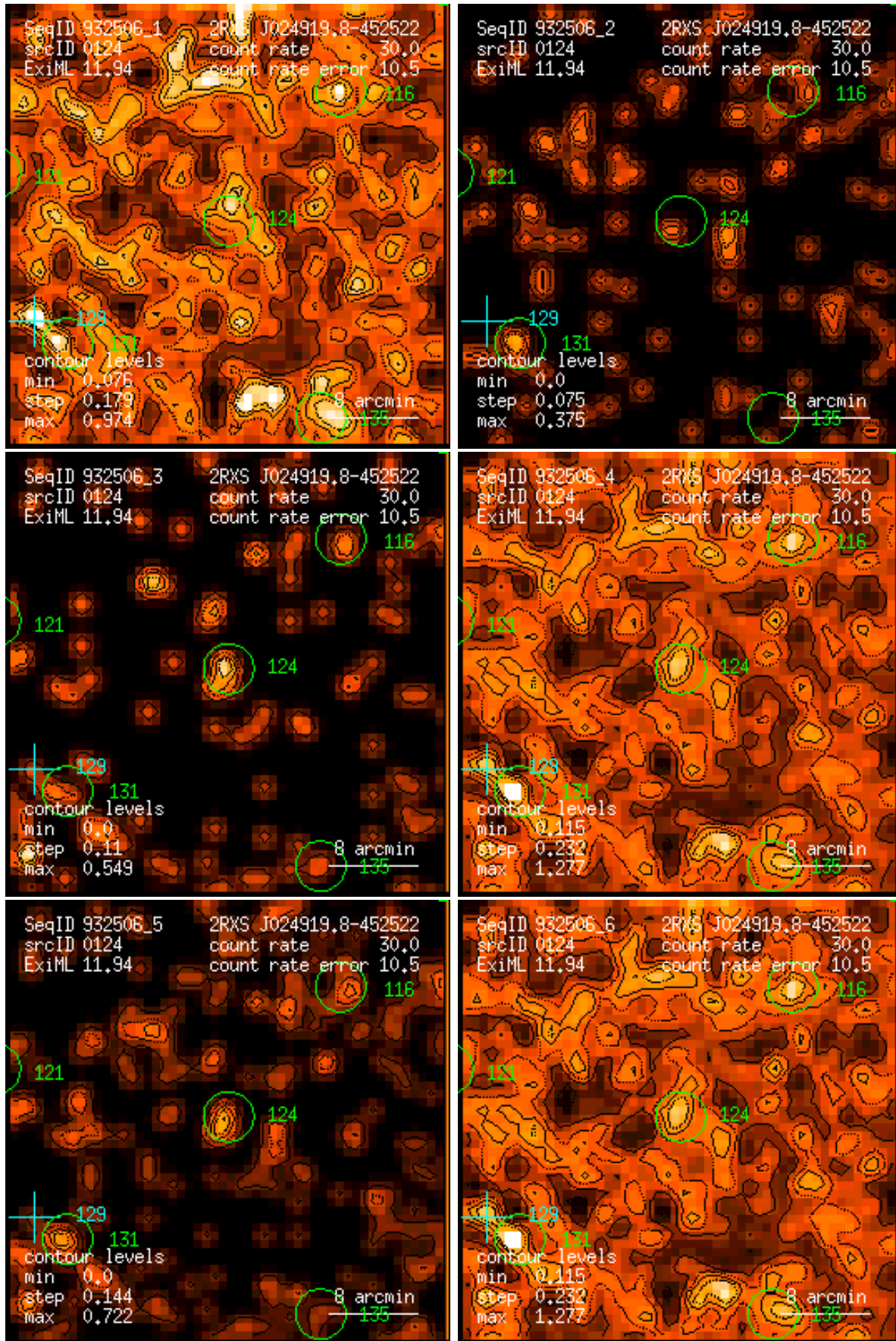
Figure 124: RASS 932506: detection 0124: band rate images, Gaussian filter: (1) PSPC channels 11 – 41, (2) 52 – 90, (3) 91 – 201, (4) 11 – 235, (5) 52 – 201, (6) 11 – 201. Broad band rates in counts/ks. Band rate contour levels in counts/ks/arcmin 2 .
