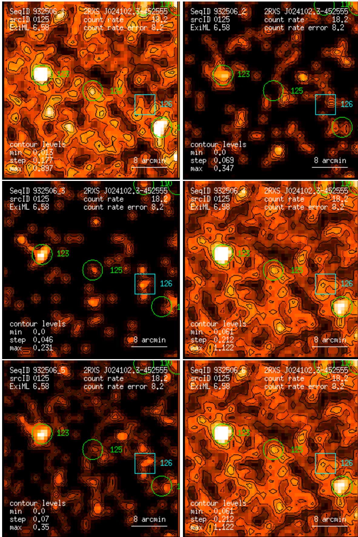
Figure 125: RASS 932506: detection 0125: band rate images, Gaussian filter: (1) PSPC channels 11 – 41, (2) 52 – 90, (3) 91 – 201, (4) 11 – 235, (5) 52 – 201, (6) 11 – 201. Broad band rates in counts/ks. Band rate contour levels in counts/ks/arcmin 2 .
