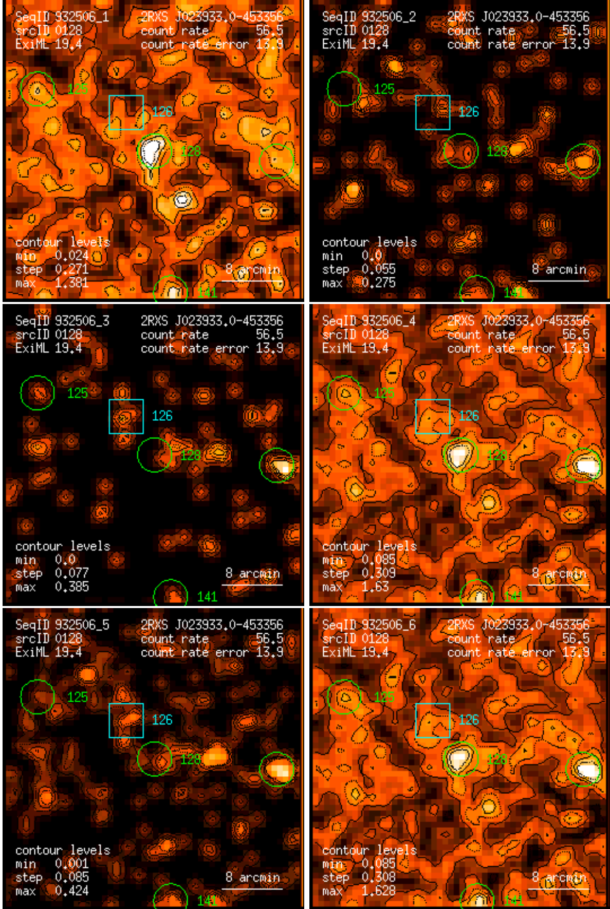
Figure 128: RASS 932506: detection 0128: band rate images, Gaussian filter: (1) PSPPC channels 11 – 41, (2) 52 – 90, (3) 91 – 201, (4) 11 – 235, (5) 52 – 201, (6) 11 – 201. Broad band rates in counts/ks. Band rate contour levels in counts/ks/arcmin 2 .
