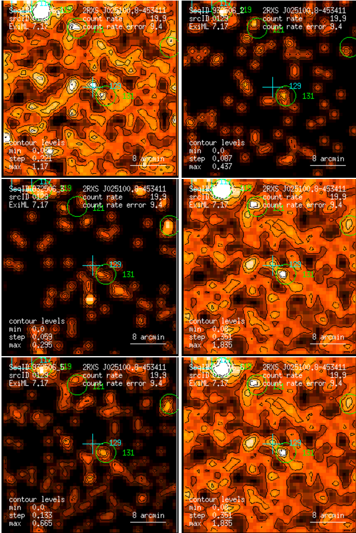
Figure 129: RASS 932506: detection 0129: band rate images, Gaussian filter: (1) PSPC channels 11 – 41, (2) 52 – 90, (3) 91 – 201, (4) 11 – 235, (5) 52 – 201, (6) 11 – 201. Broad band rates in counts/ks. Band rate contour levels in counts/ks/arcmin 2 .
