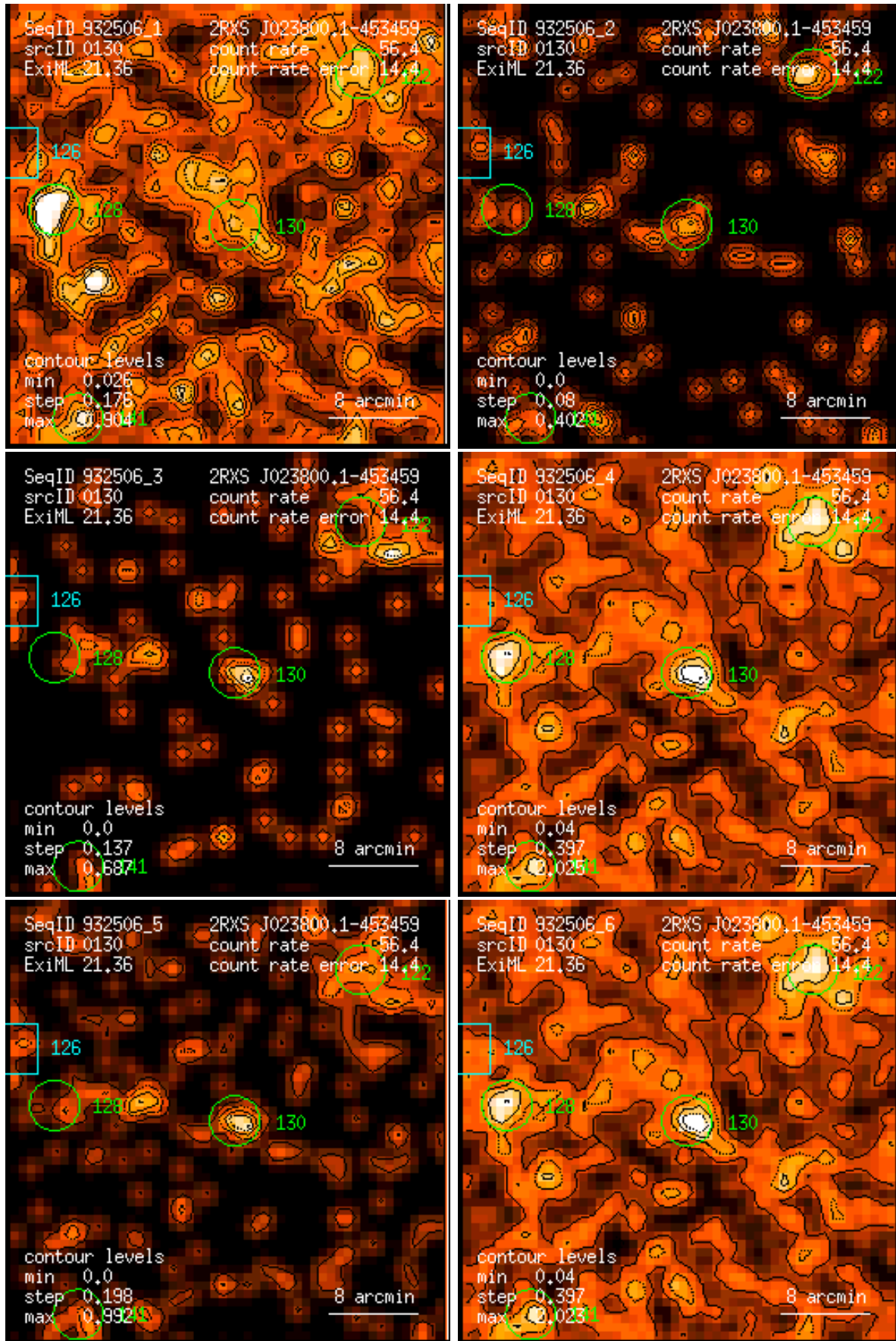
Figure 130: RASS 932506: detection 0130: band rate images, Gaussian filter: (1) PSPC channels 11 – 41, (2) 52 – 90, (3) 91 – 201, (4) 11 – 235, (5) 52 – 201, (6) 11 – 201. Broad band rates in counts/ks. Band rate contour levels in counts/ks/arcmin 2 .
