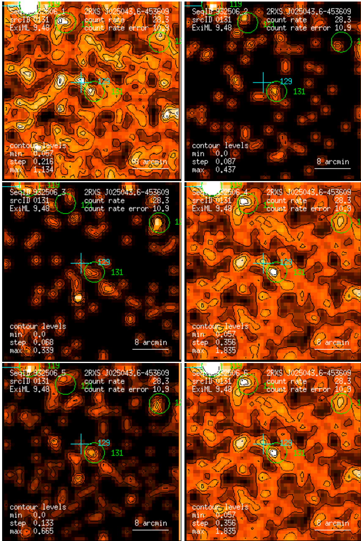
Figure 131: RASS 932506: detection 0131: band rate images, Gaussian filter: (1) PSPC channels 11 – 41, (2) 52 – 90, (3) 91 – 201, (4) 11 – 235, (5) 52 – 201, (6) 11 – 201. Broad band rates in counts/ks. Band rate contour levels in counts/ks/arcmin 2 .
