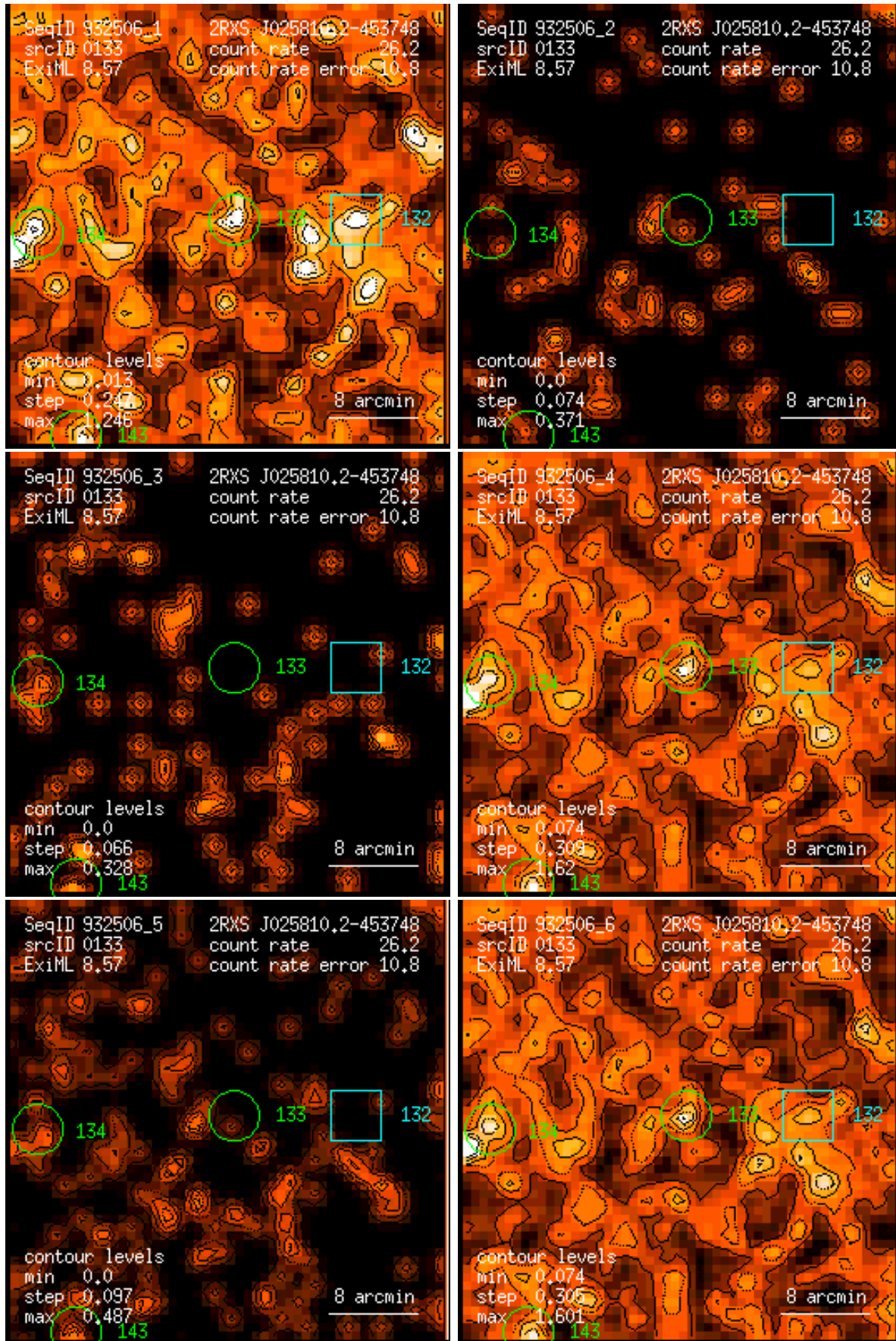
Figure 133: RASS 932506: detection 0133: band rate images, Gaussian filter: (1) PSPC channels 11 – 41, (2) 52 – 90, (3) 91 – 201, (4) 11 – 235, (5) 52 – 201, (6) 11 – 201. Broad band rates in counts/ks. Band rate contour levels in counts/ks/arcmin 2 .
