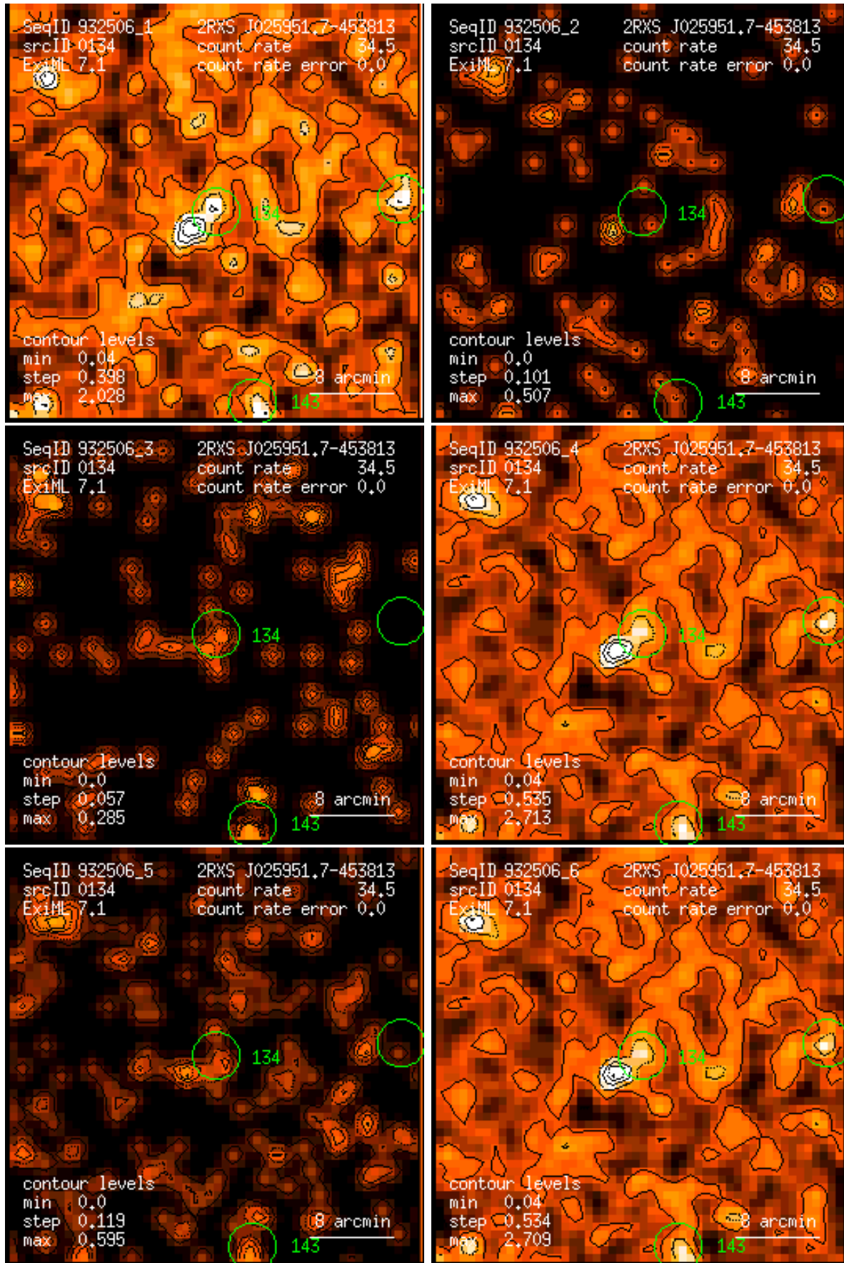
Figure 134: RASS 932506: detection 0134: band rate images, Gaussian filter: (1) PSPC channels 11 – 41, (2) 52 – 90, (3) 91 – 201, (4) 11 – 235, (5) 52 – 201, (6) 11 – 201. Broad band rates in counts/ks. Band rate contour levels in counts/ks/arcmin 2 .
