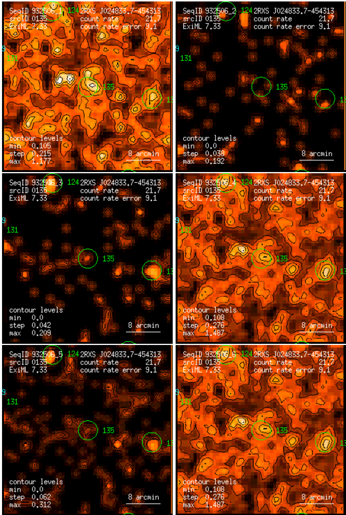
Figure 135: RASS 932506: detection 0135: band rate images, Gaussian filter: (1) PSPC channels 11 – 41, (2) 52 – 90, (3) 91 – 201, (4) 11 – 235, (5) 52 – 201, (6) 11 – 201. Broad band rates in counts/ks. Band rate contour levels in counts/ks/arcmin 2 .
