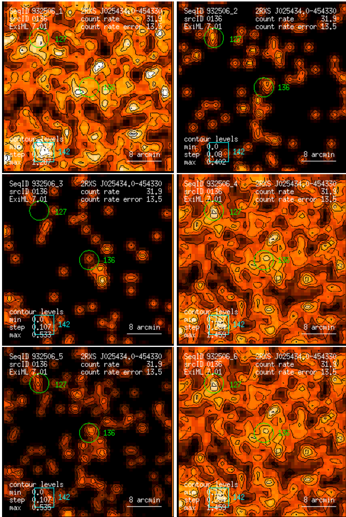
Figure 136: RASS 932506: detection 0136: band rate images, Gaussian filter: (1) PSPC channels 11 – 41, (2) 52 – 90, (3) 91 – 201, (4) 11 – 235, (5) 52 – 201, (6) 11 – 201. Broad band rates in counts/ks. Band rate contour levels in counts/ks/arcmin 2 .
