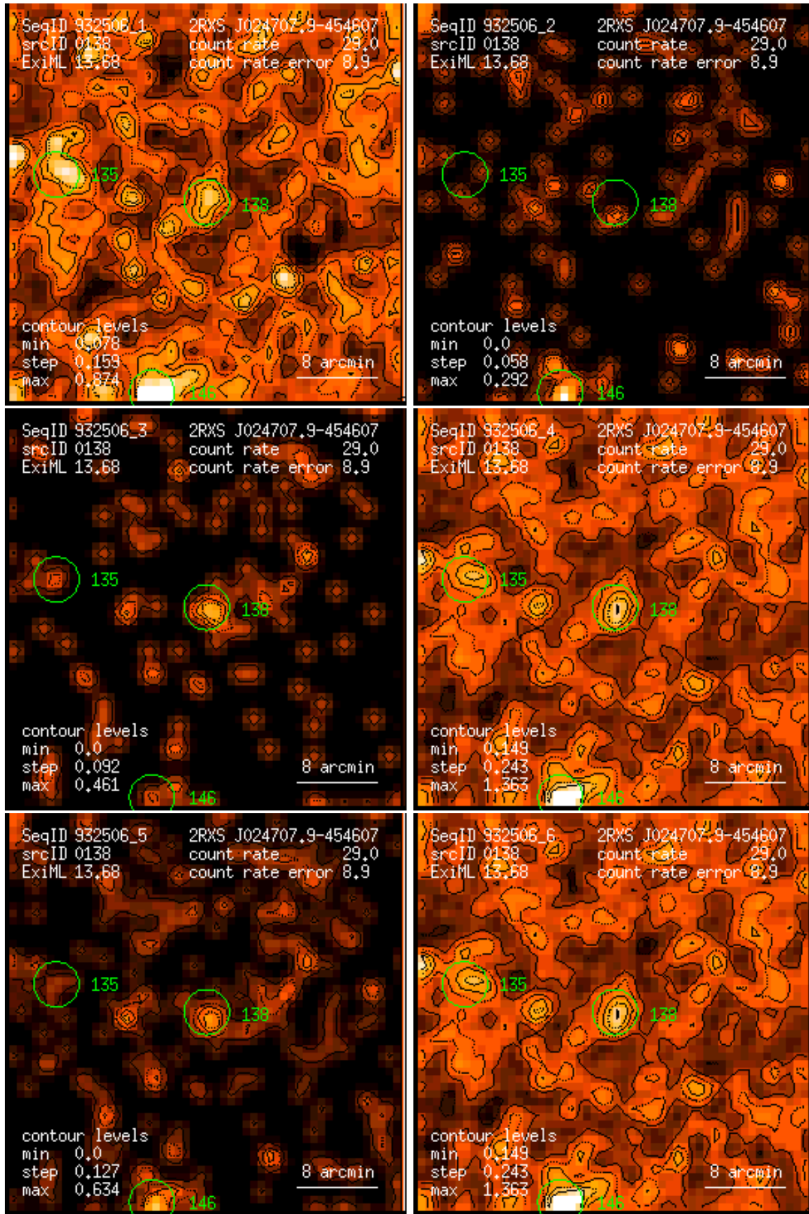
Figure 138: RASS 932506: detection 0138: band rate images, Gaussian filter: (1) PSPC channels 11 – 41, (2) 52 – 90, (3) 91 – 201, (4) 11 – 235, (5) 52 – 201, (6) 11 – 201. Broad band rates in counts/ks. Band rate contour levels in counts/ks/arcmin 2 .
