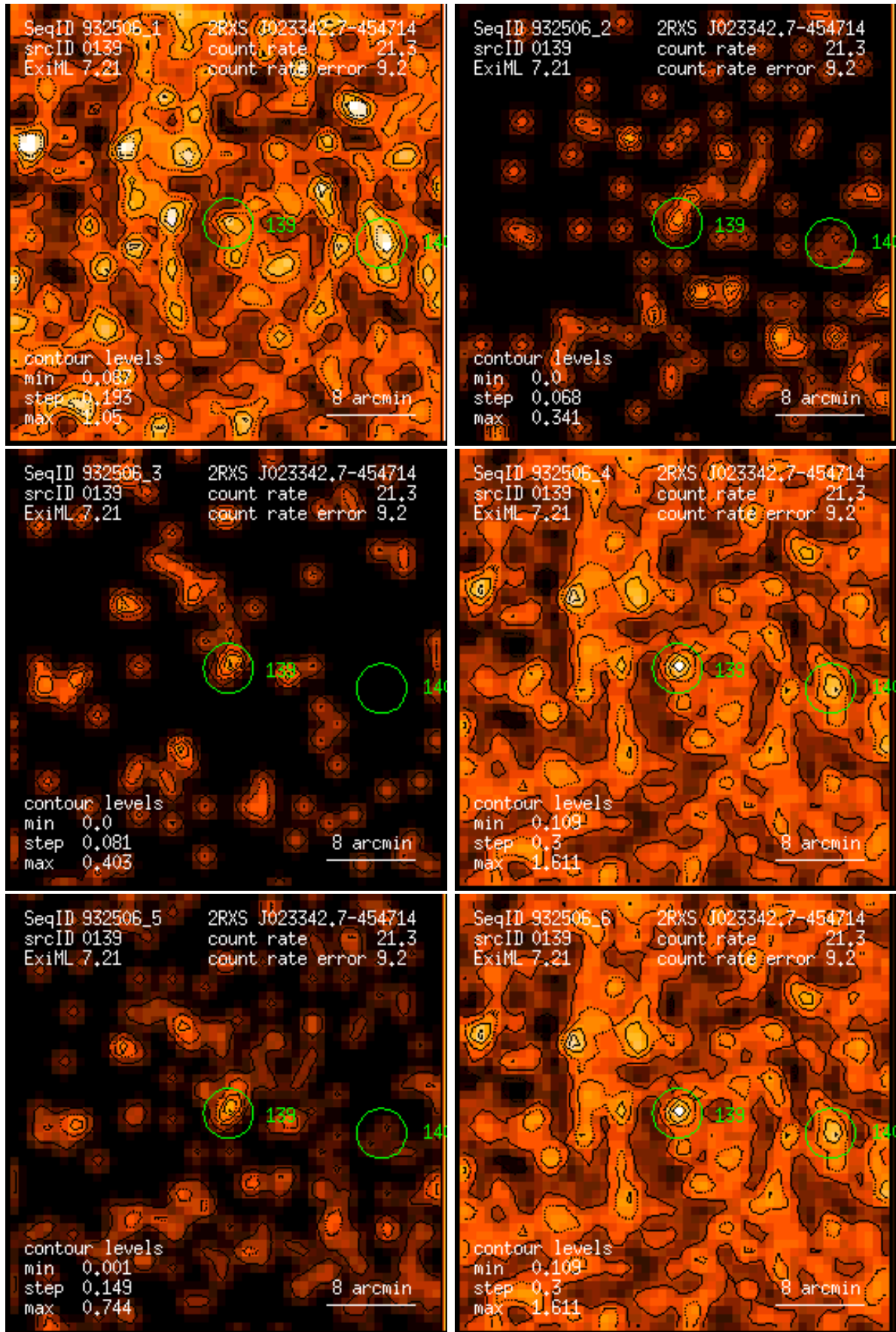
Figure 139: RASS 932506: detection 0139: band rate images, Gaussian filter: (1) PSPC channels 11 – 41, (2) 52 – 90, (3) 91 – 201, (4) 11 – 235, (5) 52 – 201, (6) 11 – 201. Broad band rates in counts/ks. Band rate contour levels in counts/ks/arcmin 2 .
