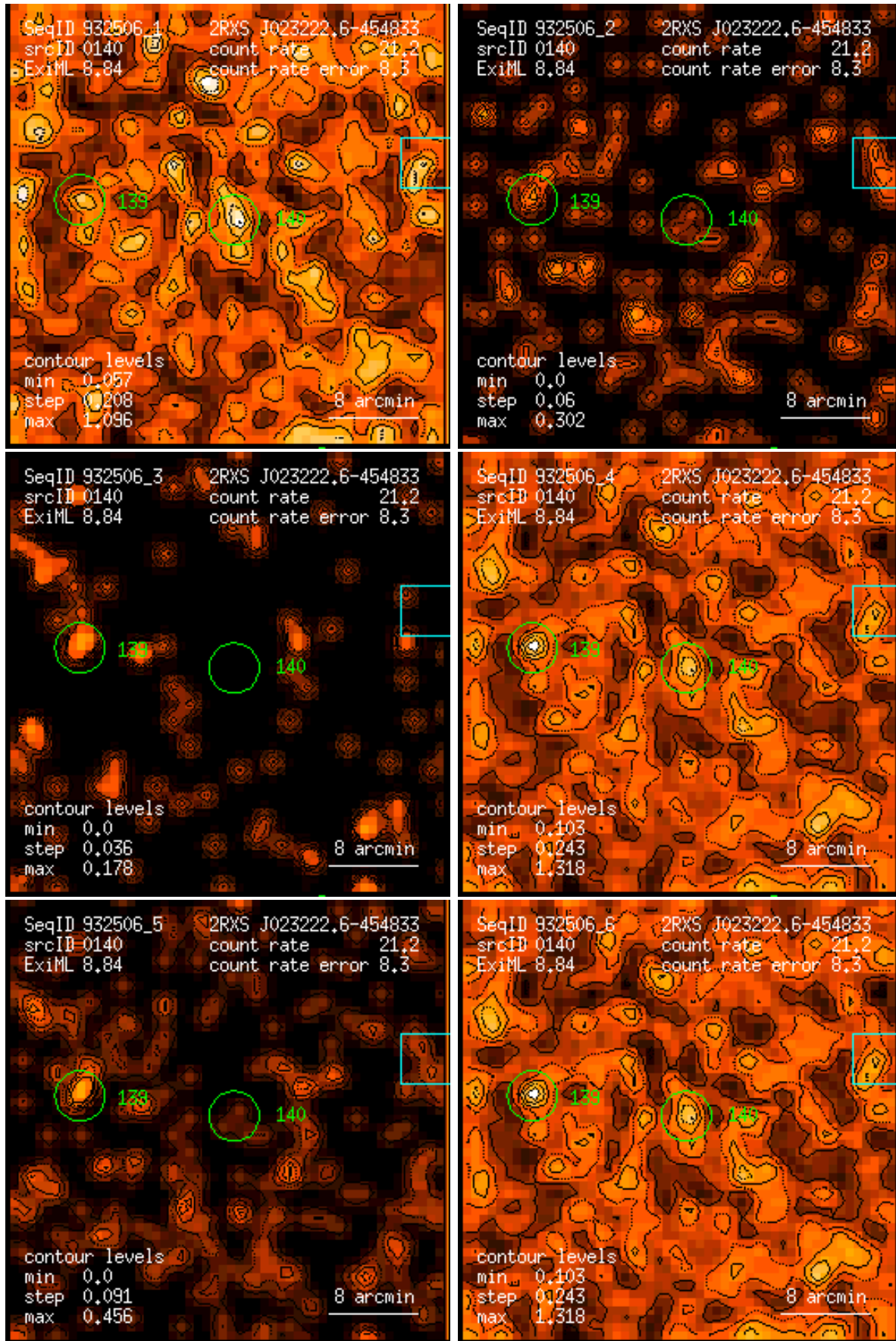
Figure 140: RASS 932506: detection 0140: band rate images, Gaussian filter: (1) PSPC channels 11 – 41, (2) 52 – 90, (3) 91 – 201, (4) 11 – 235, (5) 52 – 201, (6) 11 – 201. Broad band rates in counts/ks. Band rate contour levels in counts/ks/arcmin 2 .
