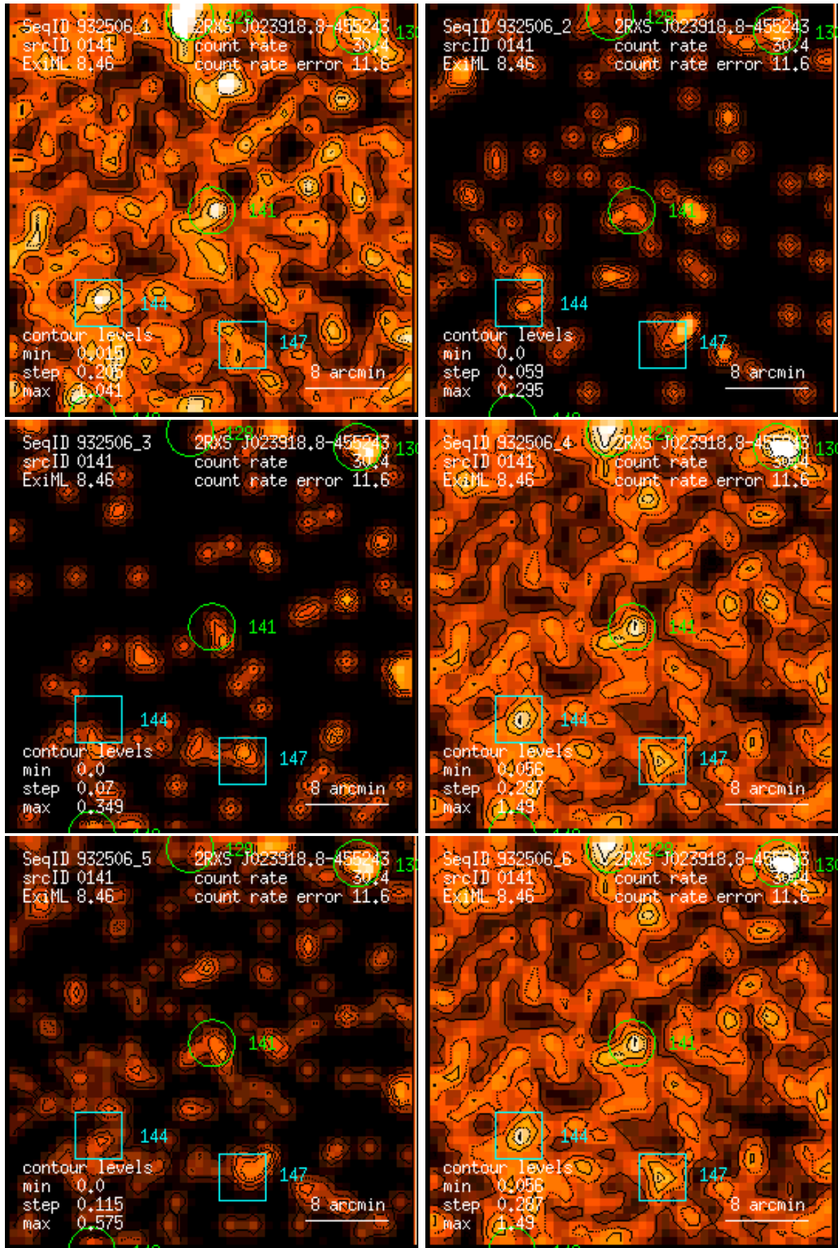
Figure 141: RASS 932506: detection 0141: band rate images, Gaussian filter: (1) PSPC channels 11 – 41, (2) 52 – 90, (3) 91 – 201, (4) 11 – 235, (5) 52 – 201, (6) 11 – 201. Broad band rates in counts/ks. Band rate contour levels in counts/ks/arcmin 2 .
