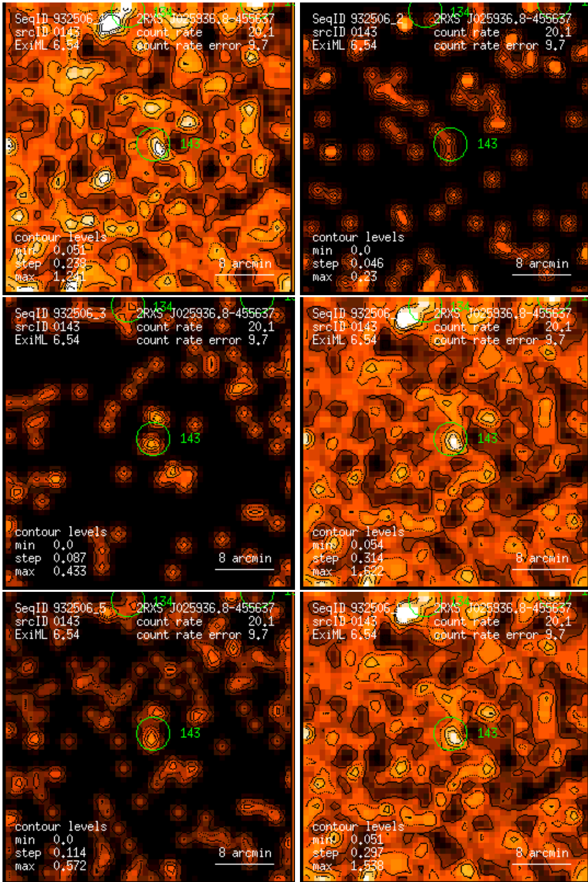
Figure 143: RASS 932506: detection 0143: band rate images, Gaussian filter: (1) PSPC channels 11 – 41, (2) 52 – 90, (3) 91 – 201, (4) 11 – 235, (5) 52 – 201, (6) 11 – 201. Broad band rates in counts/ks. Band rate contour levels in counts/ks/arcmin 2 .
