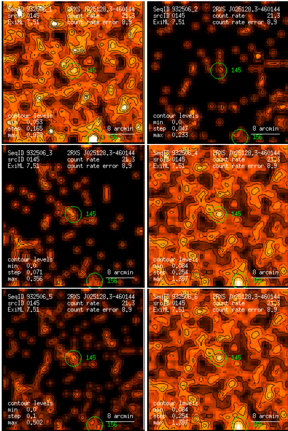
Figure 145: RASS 932506: detection 0145: band rate images, Gaussian filter: (1) PSPC channels 11 – 41, (2) 52 – 90, (3) 91 – 201, (4) 11 – 235, (5) 52 – 201, (6) 11 – 201. Broad band rates in counts/ks. Band rate contour levels in counts/ks/arcmin 2 .
